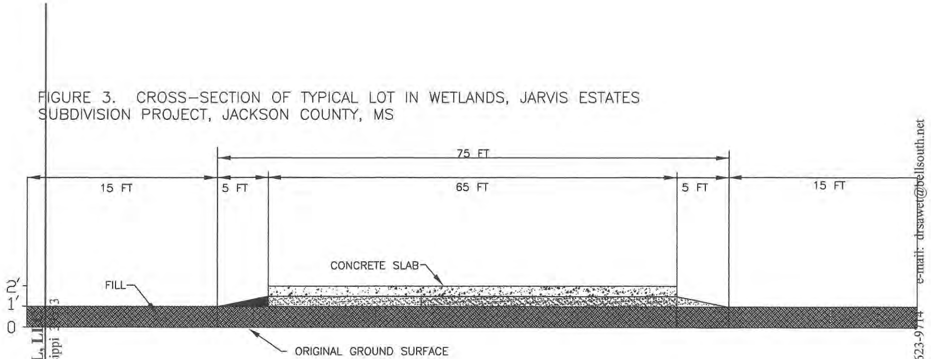
CROSS-SECTION OF TYPICAL LOT IN WETLANDS (VERTICAL SCALE IN FEET ABOVE GROUND SURFACE)
