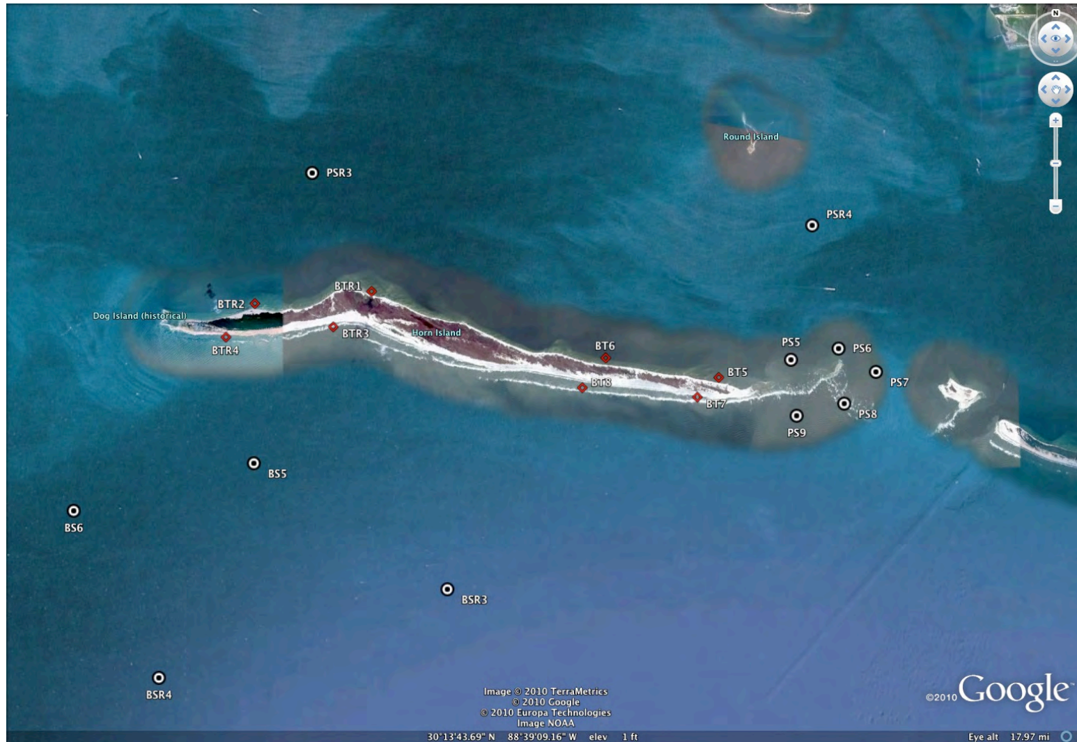
Figure 3. Horn Island station locations for the Benthic Macroinfaunal Community Assessment, MsCIP, 2010 - 2011.
