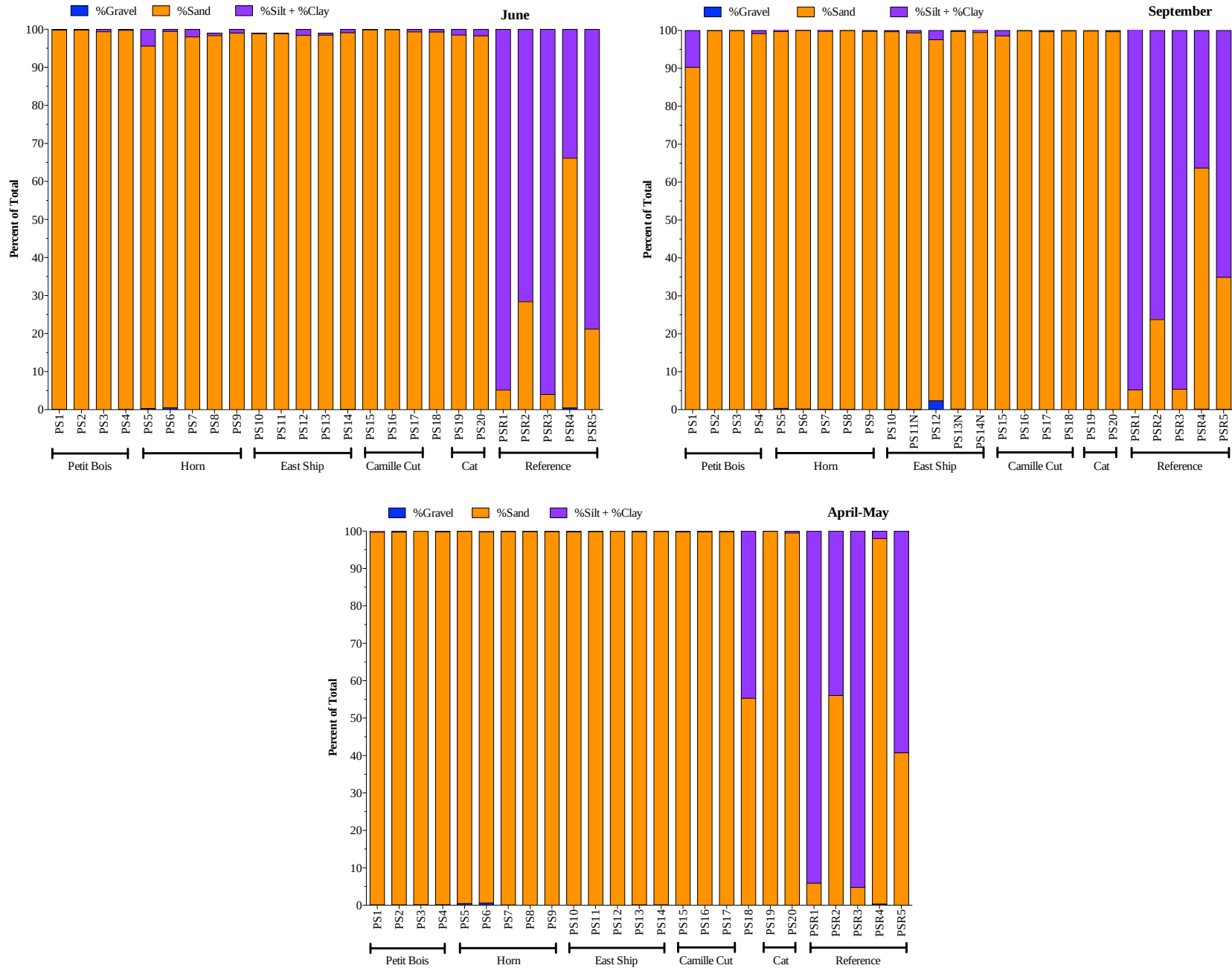
Figure 17. Sediment texture data for the MsCIP Placement Site stations, June 2010, September 2010, and April-May 2011.
