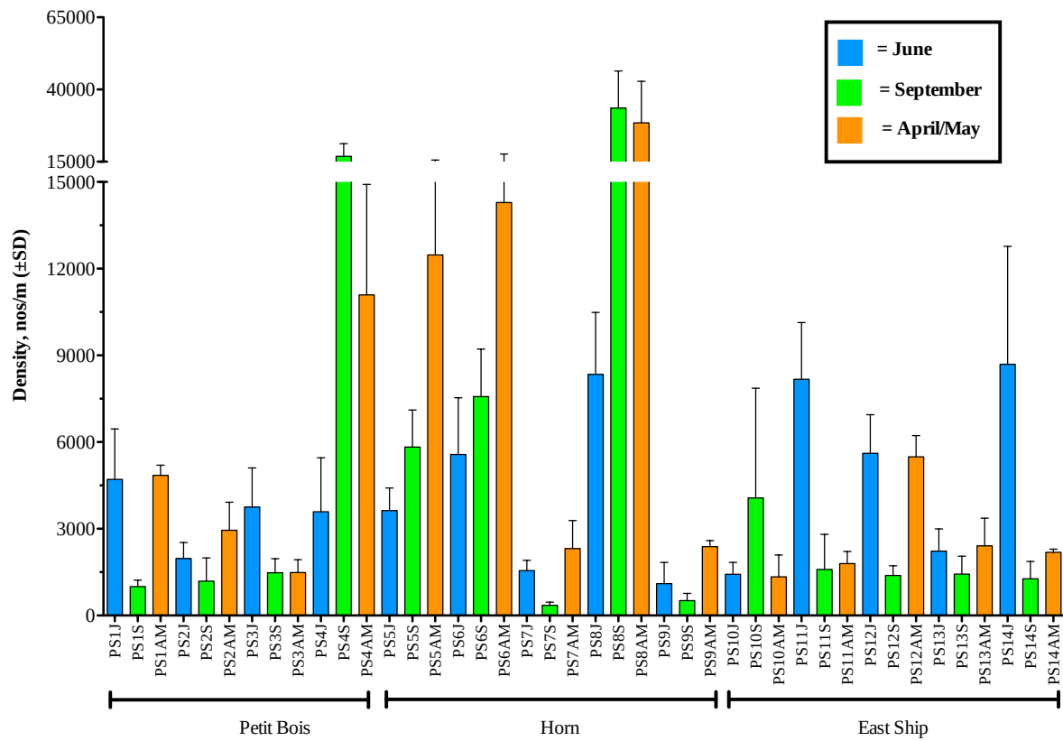
Figure 24. Density data for the Placement Site stations June 2010, September 2010 and April-May 2011.
