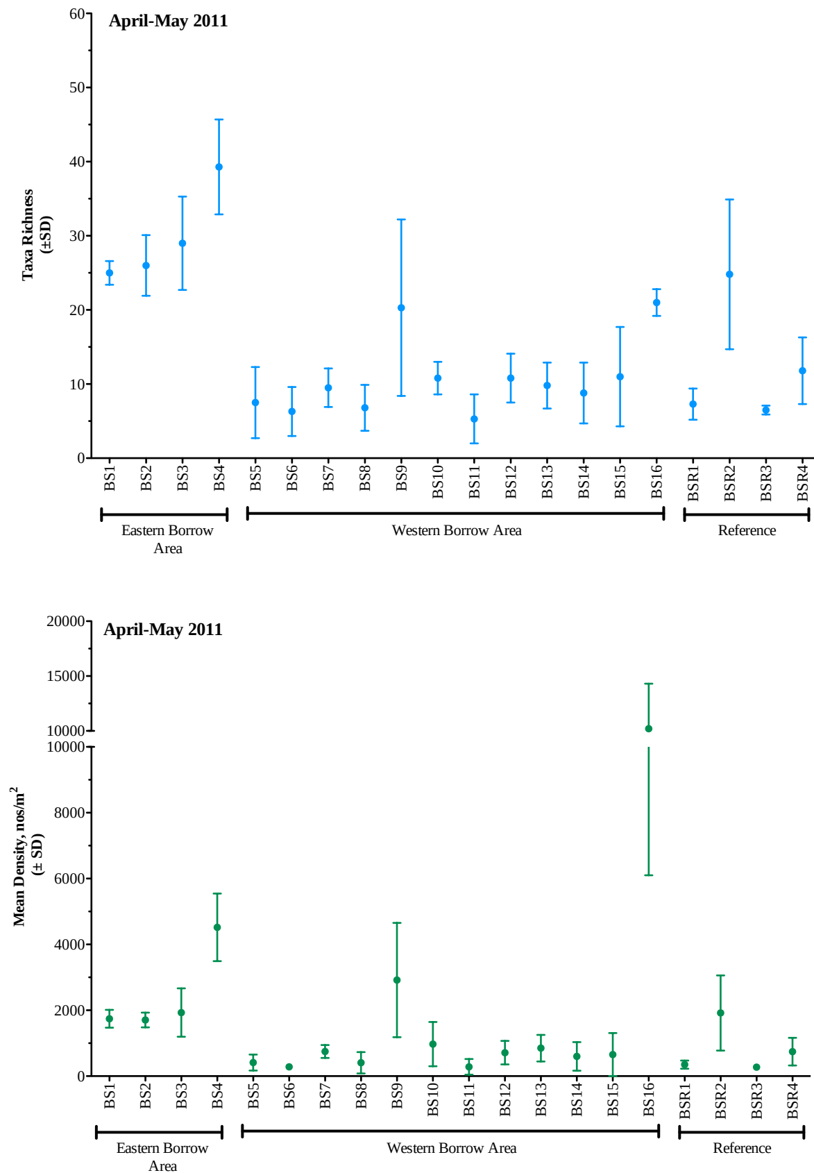
Figure 13. Taxa richness and density data for the MsCIP Borrow Site stations, April-May 2011.
