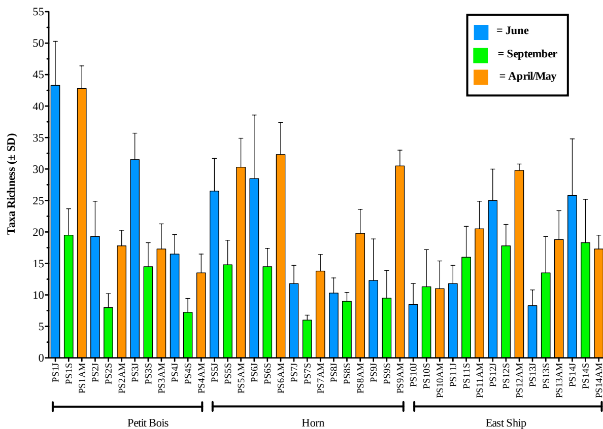
Figure 23. Taxa richness data for the Placement Site stations June 2010, September 2010 and April-May 2011.
