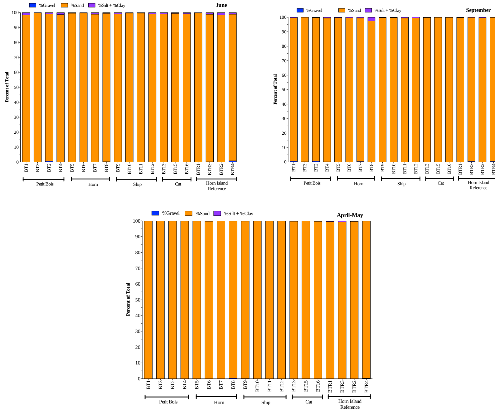
Figure 27. Sediment texture data for the MsCIP Beach Transect Shallow stations, June 2010, September 2010 and April-May 2011.
