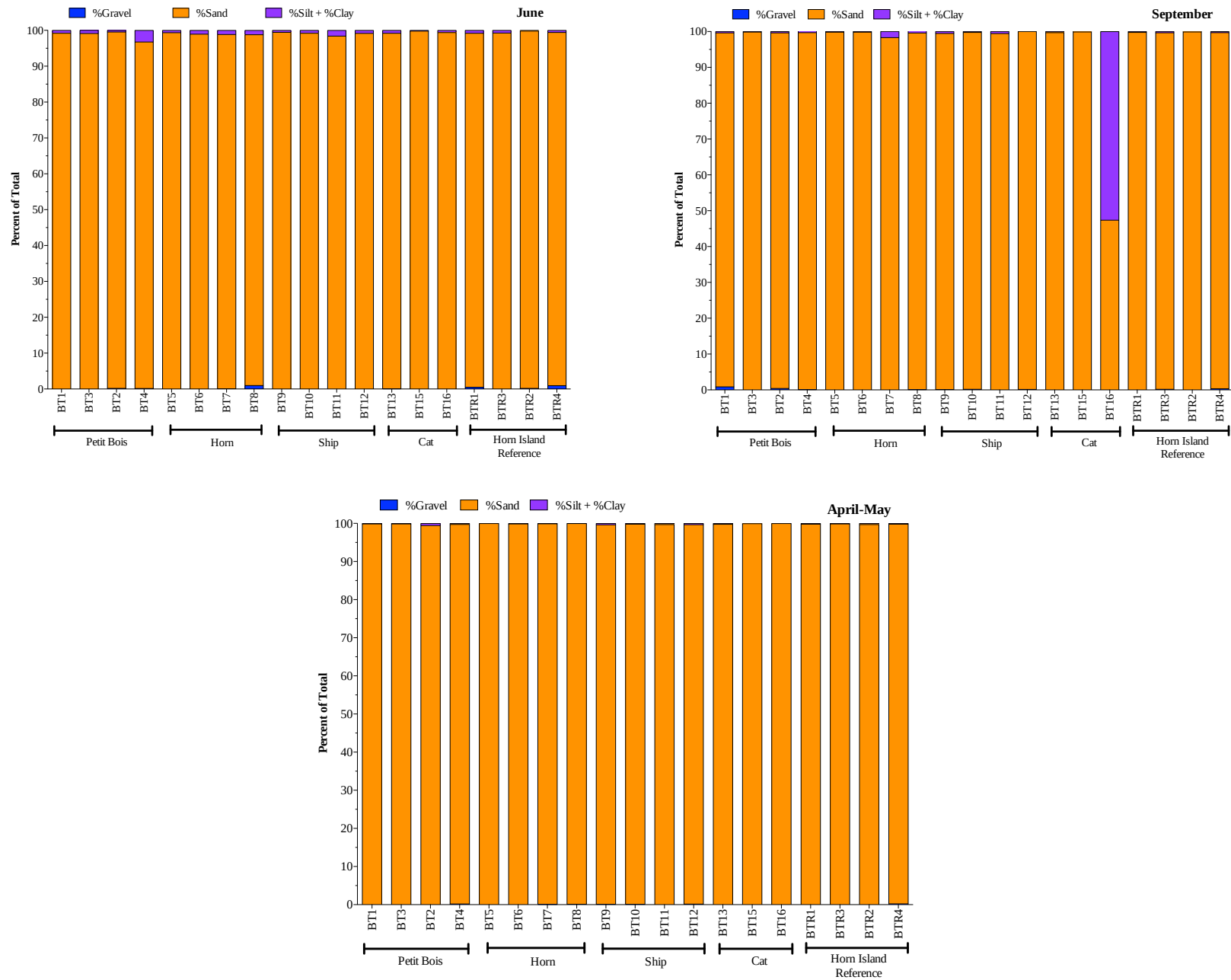
Figure 28. Sediment texture data for the MsCIP Beach Transect Mid-Depth stations, June 2010, September 2010 and April-May 2011.
