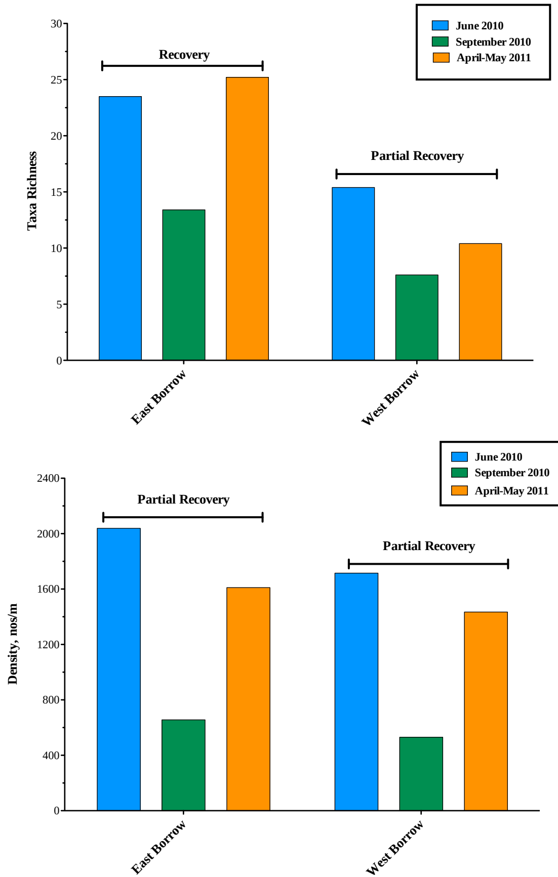
Figure 51. A summary of taxa richness and density for the Borrow Site Stations.
