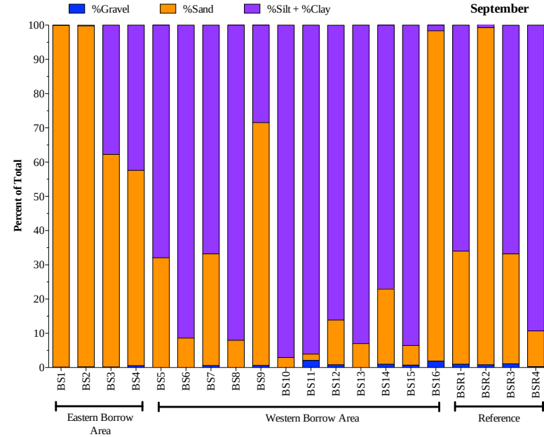
Figure 6. Sediment texture data for the MsCIP Borrow Site stations, June and September 2010, and April-May 2011.
