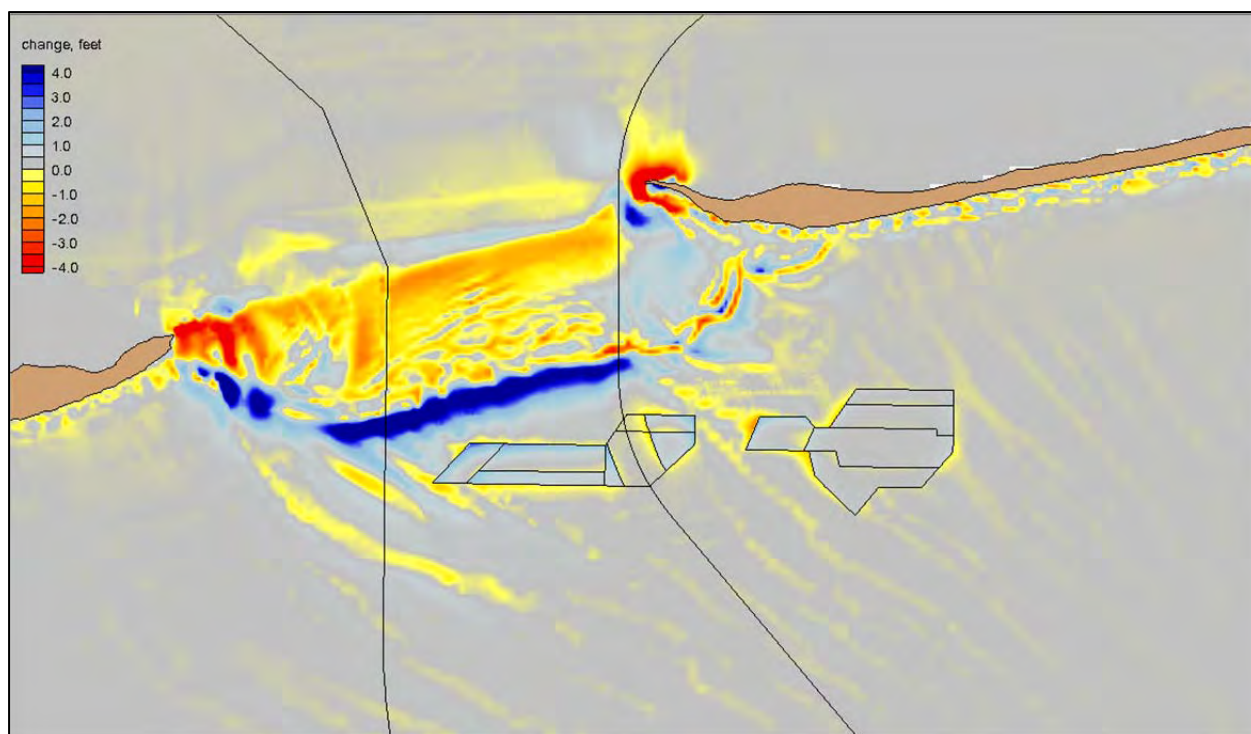
Figure 42. Contour map of bathymetric change for post-dredging conditions at the Petit Bois borrow sites from the year-long simulation. Borrow site boundaries and pipelines also are shown.
