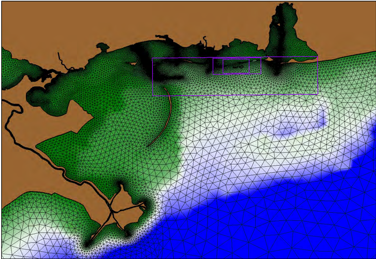
Figure 28. Close up of GoM ADCIRC grid with purple colored outlines denoting the CMS-Wave and Flow grid extents.
