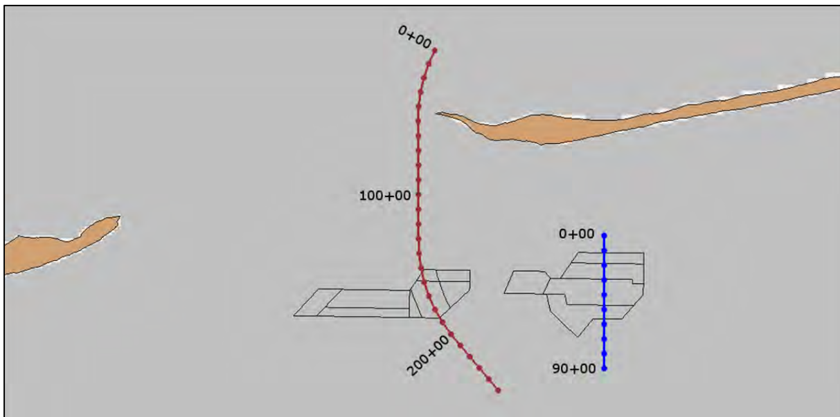
Figure 34. Transects used to plot morphology data across borrow sites. The blue transect that cross PBW follows the lay of the Gulfstream pipeline. Markers along lines are spaced every 1000 feet. Stationing is also provided in feet.
