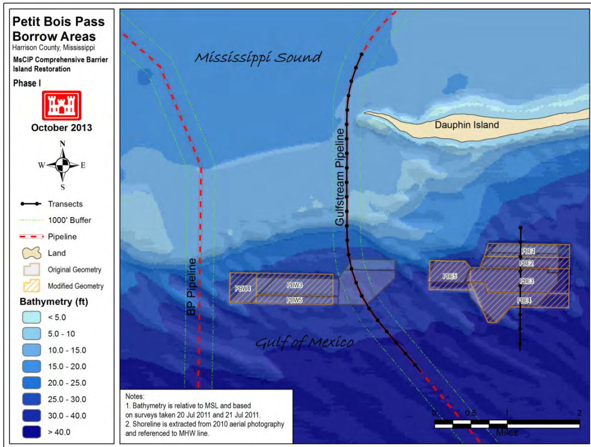
Figure 1: Petit Bois Pass borrow area geometry modification in response to Gulfstream pipeline owner's concerns.
