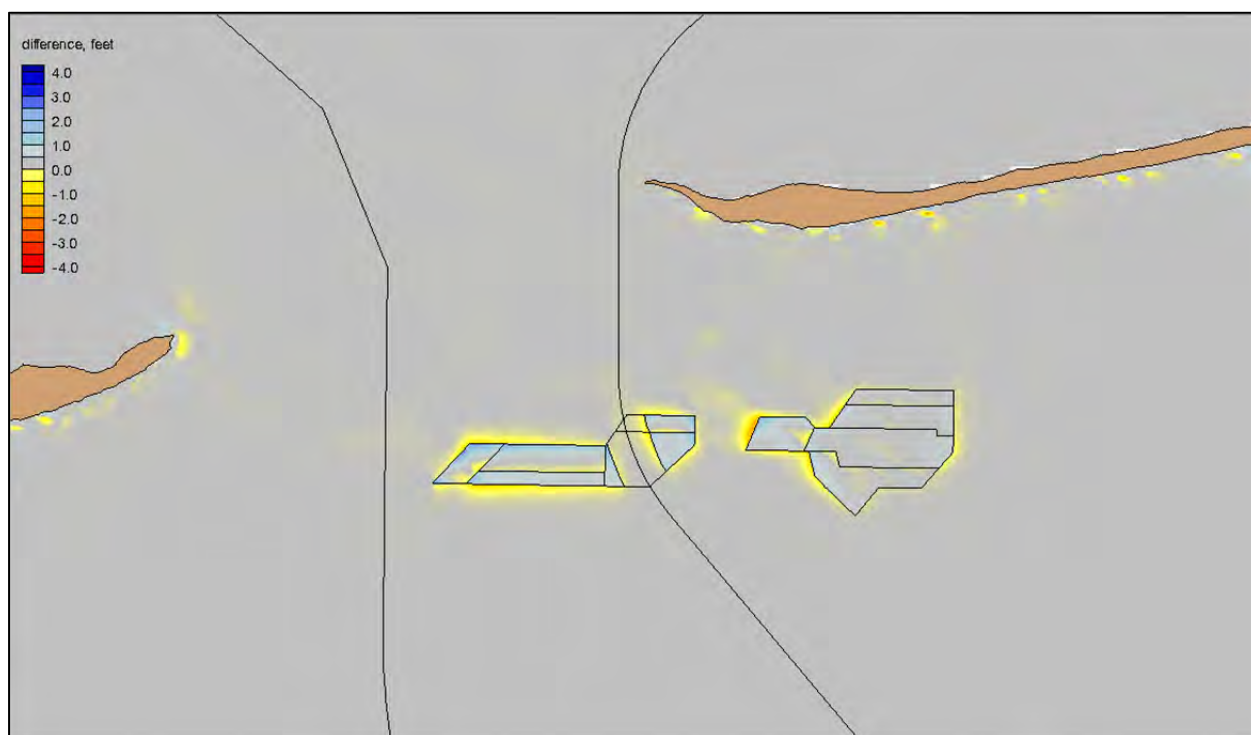
Figure 43. Difference map for existing and post-dredging morphology change from simulations of annual conditions.
