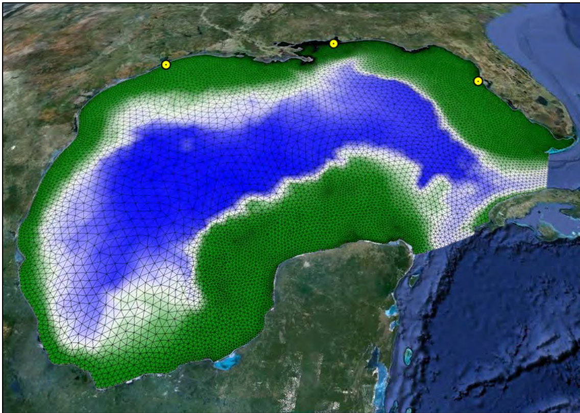
Figure 27. ADCIRC mesh of the Gulf of Mexico, showing grid elements and color contours overlaid on the Google Earth terrain map of the globe. NOAA tide stations used to calibrate the model are indicated by yellow markers (Galveston, TX; Dauphin Is., AL; Clearwater Beach, FL from west to east).
