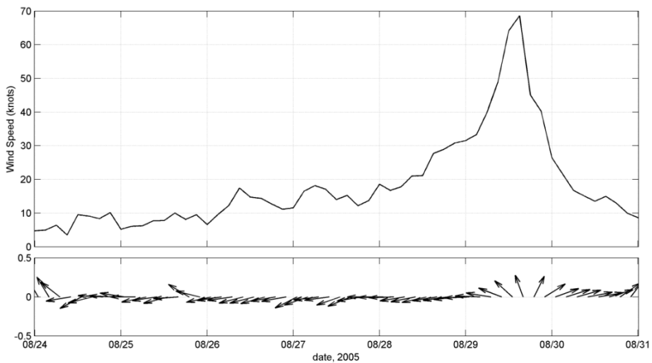
Figure 26. Plot of wind speed and direction during Hurricane Katrina from the Oceanweather storm hindcast. Vectors indicate compass direction to where the wind was blowing.
