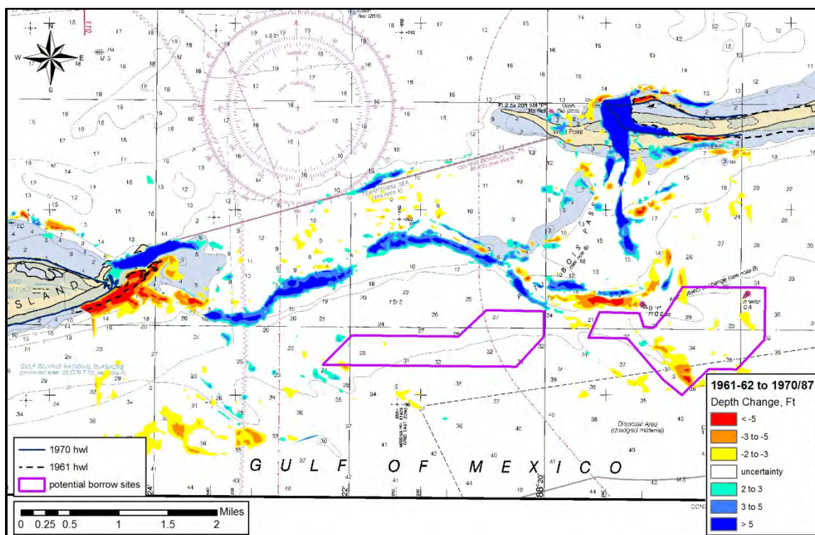
Figure 17. Bathymetric change between 1961-62 and 1970/87 for Petit Bois Pass.
