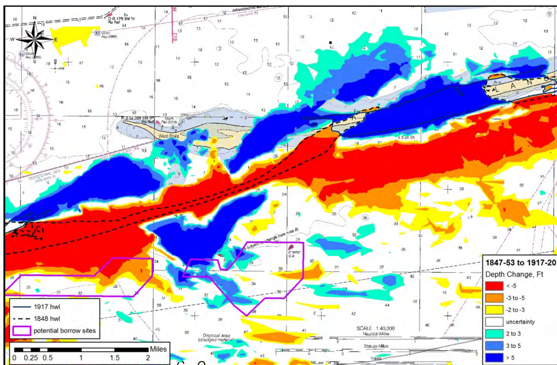
Figure 15. Bathymetric change between 1847-53 and 1917-20 for Petit Bois Pass.
