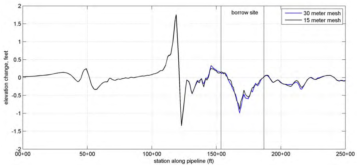
Figure 35. Comparison of simulations of Hurricane Katrina, run with two CMS-Flow meshes; a mesh with a 30 m minimum cell size (blue line) and a 15 m minimum cell size (black line). Output is provided along a segment of the Gulfstream pipeline shown in Figure 34.
