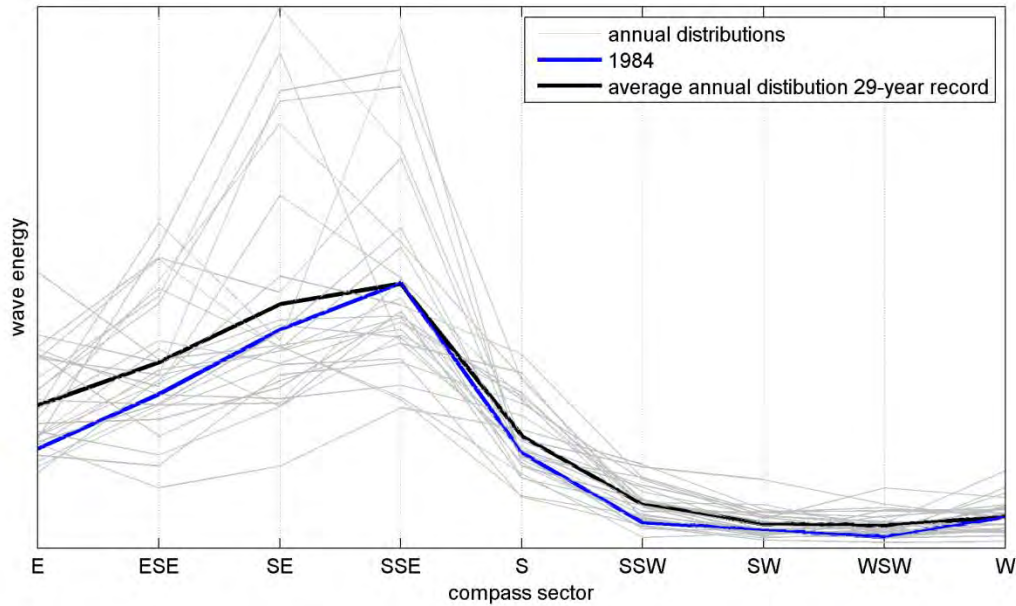
Figure 23. Distribution of total wave energy by compass sector from the OWI 29-year hindcast. Annual sums of wave energy (grey lines) are compared to the average for the entire record by sector (black line). The year with the best comparison to the entire record (1984) is indicated using a blue line.
