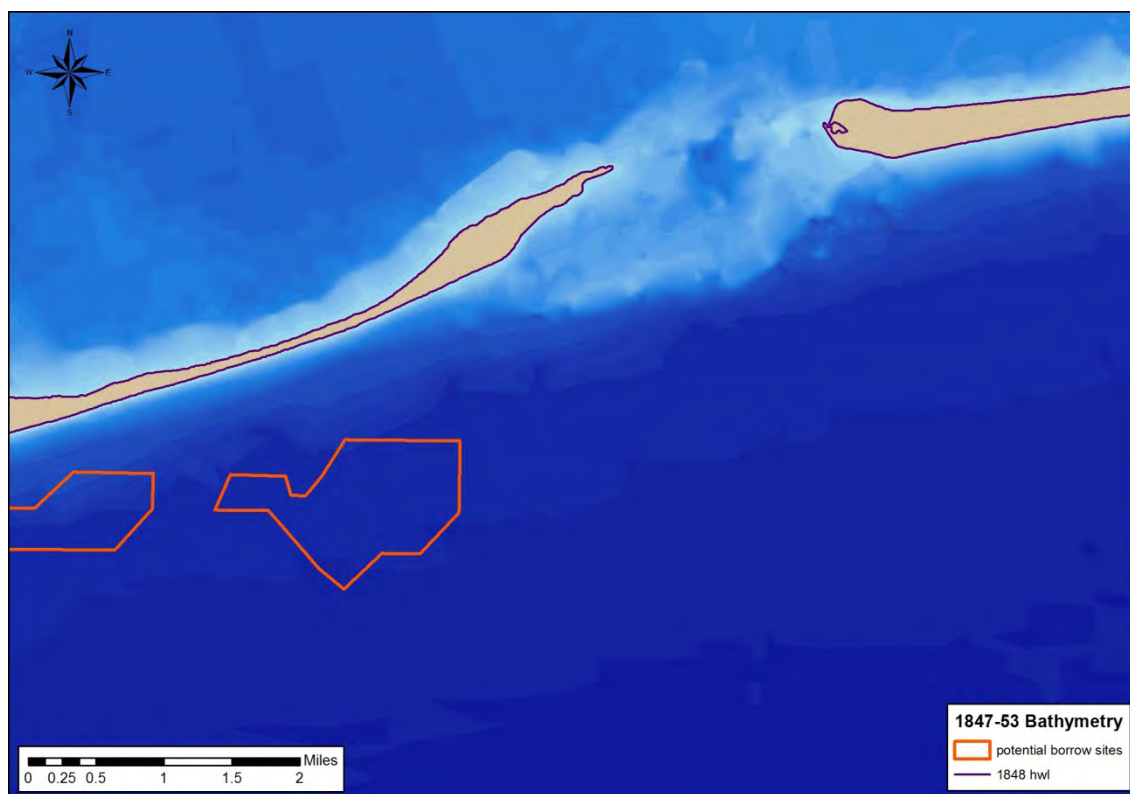
Figure 8. Bathymetric surface for Petit Bois Pass, 1847-53.
