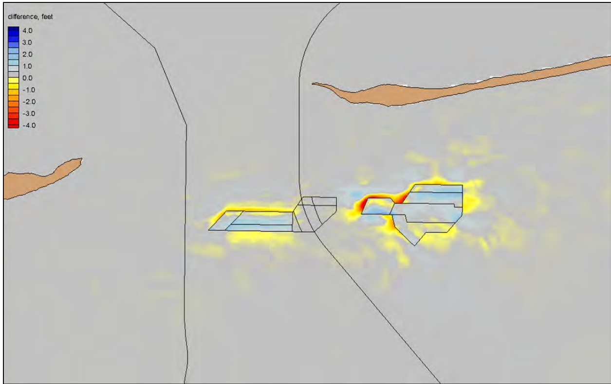
Figure 50. Difference between existing and modified post-dredging (no dredging of PBW1 and PBW2) morphology change from simulations of storm conditions.
