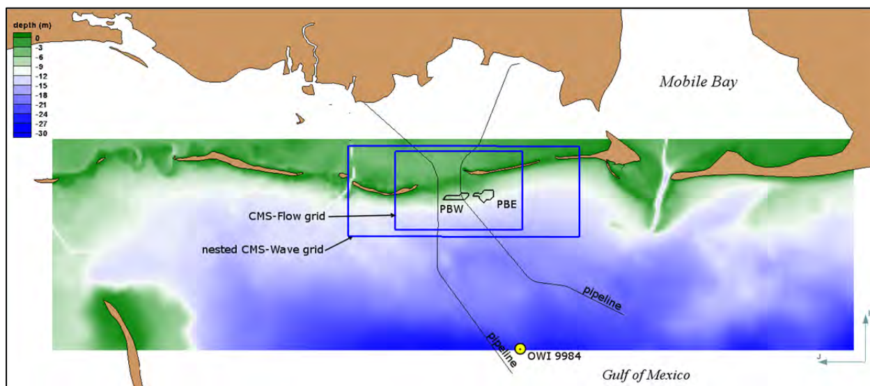
Figure 21. Map showing extent of CMS-Wave coarse grid with color-shaded bathymetric contours. The extents of the nested CMS-Wave grid of Petit Bois Pass and the CMS-Flow grid are indicated by blue rectangles. Paths of the two pipelines that traverse Petit Bois Pass are illustrated.
