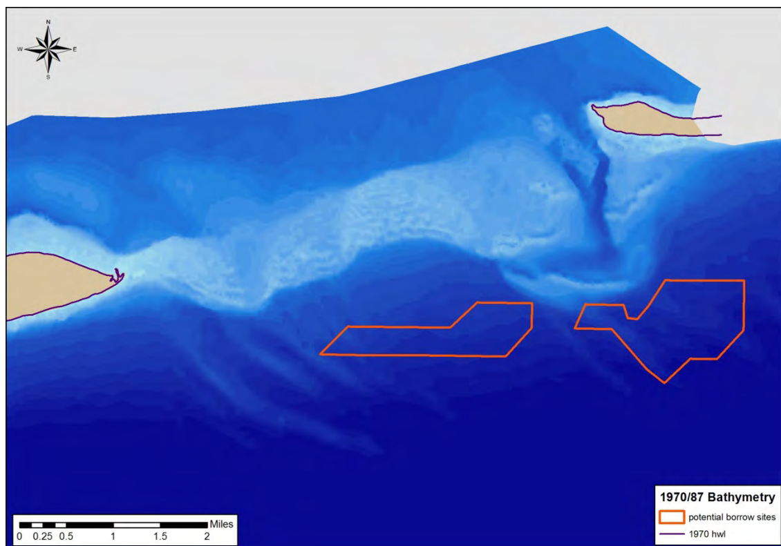
Figure 11. Bathymetric surface for Petit Bois Pass, 1970/87.
