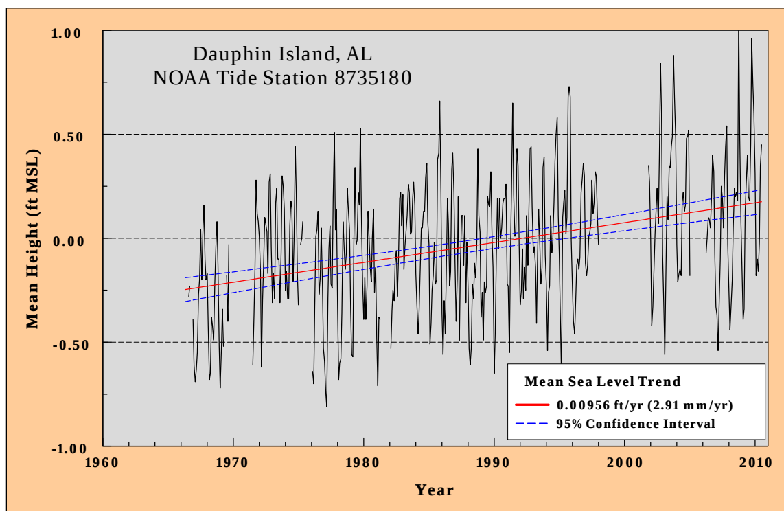
Figure 7. Monthly mean water level measurements and sea-level rise trend at Dauphin Island, AL gauge 8735180, 1966 to 2010.
