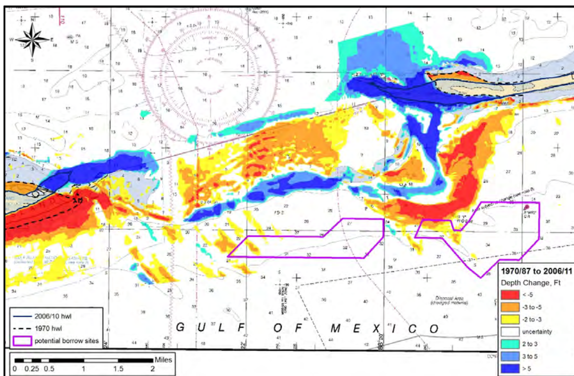
Figure 18. Bathymetric change between 1970/87 and 2006/11 for Petit Bois Pass.
