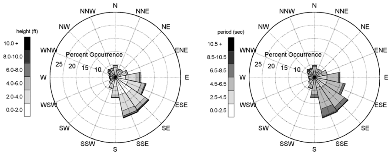
Figure 20. Wave height and period for Oceanweather, Inc hindcast grid point 9984 (14 NM south of Dauphin Island) for the 29-year period between January 1980 and December 2008. Direction indicates from where waves were traveling, relative to true north. Radial length of gray tone segments indicates percent occurrence for each range of wave heights and periods. Combined length of segments in each sector indicate percent occurrence of all waves from that direction.
