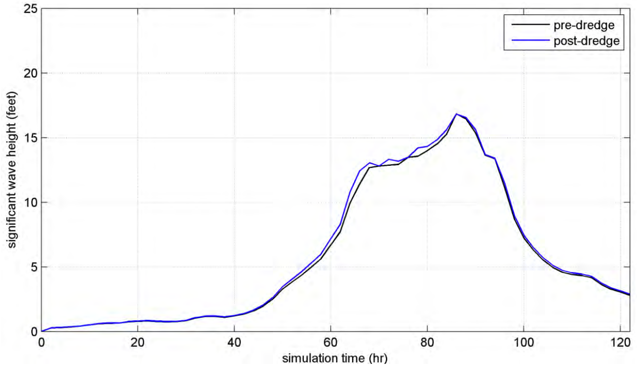
Figure 38. Plot of model wave height at the point where the Gulfstream pipeline intersects the northern boundary of PBW for existing and post-dredging conditions at the borrow site.
