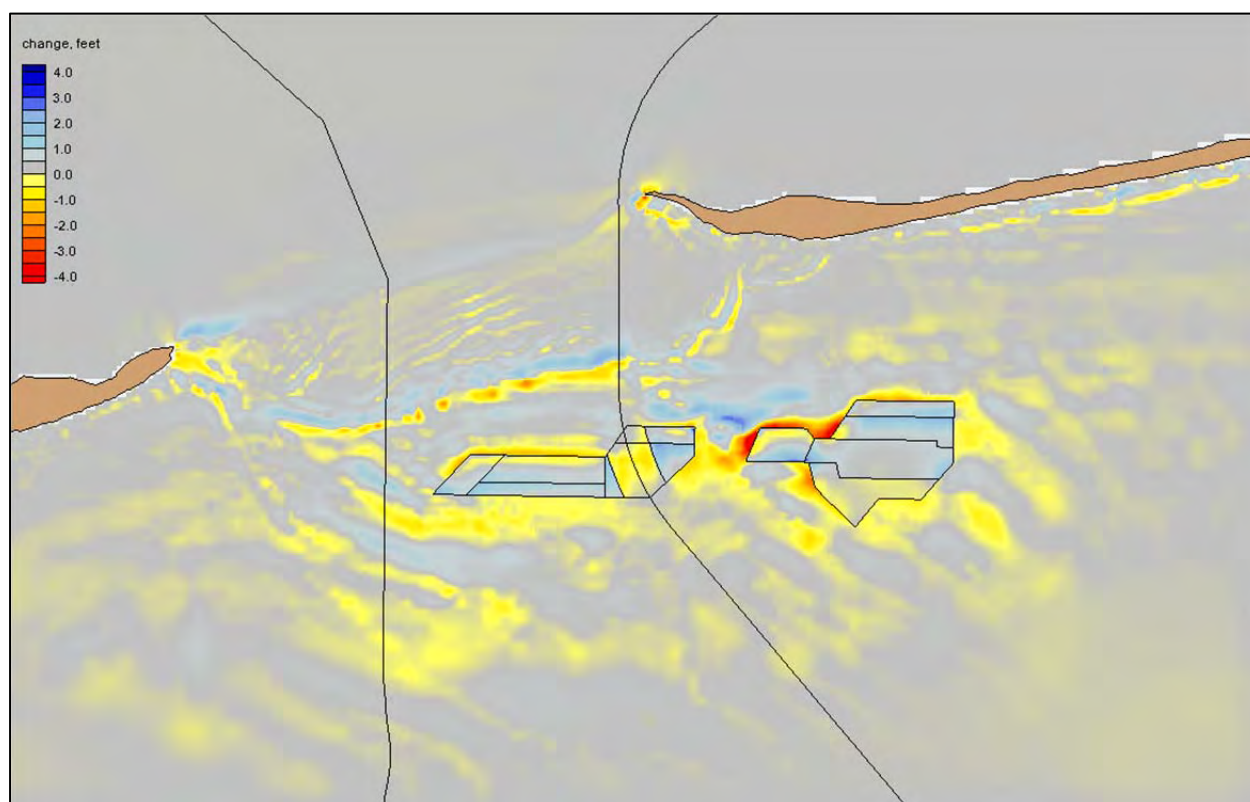
Figure 44. Contour map of bathymetric change for post-dredging conditions at the Petit Bois borrow sites from the simulation of Hurricane Katrina. Borrow site boundaries and pipelines also are shown.
