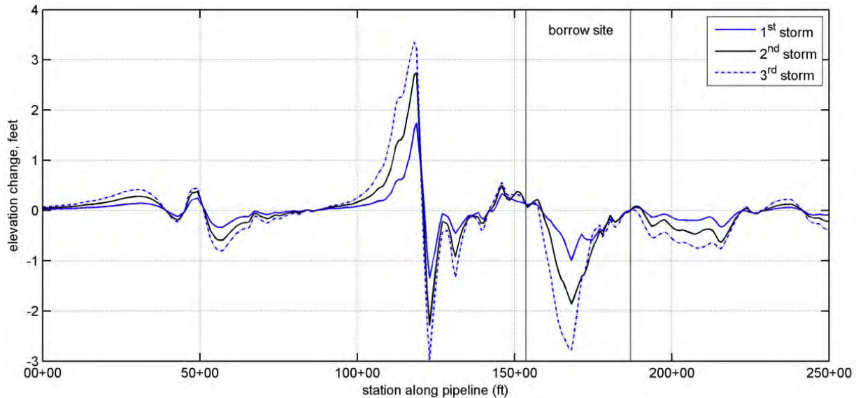
Figure 47. Cumulative morphology change along the Gulfstream pipeline transect (Figure 34) resulting from three Hurricane Katrina scale storms.
