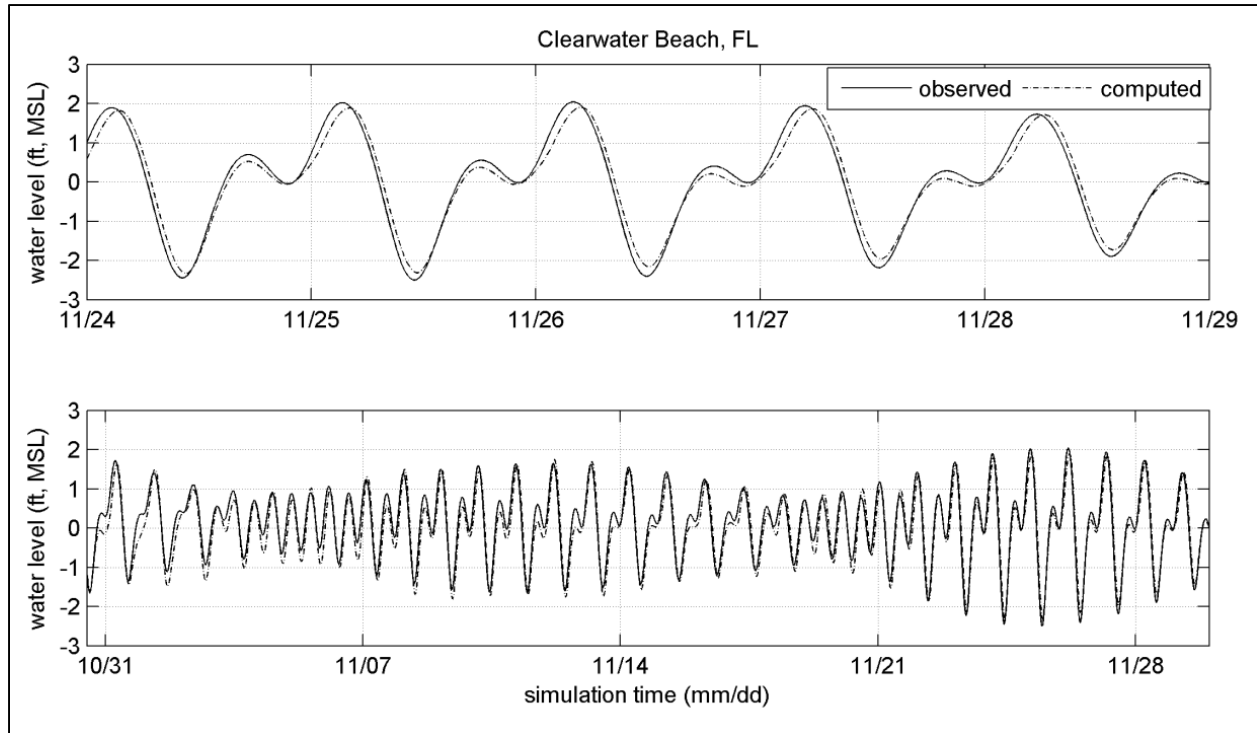
Figure 31. Comparison of modeled and NOAA predicted tide at Clearwater Beach, FL. R2 correlation is 0.90 and RMS error is 0.2 feet. The top plot is a subset of the complete month shown in the bottom plot.
