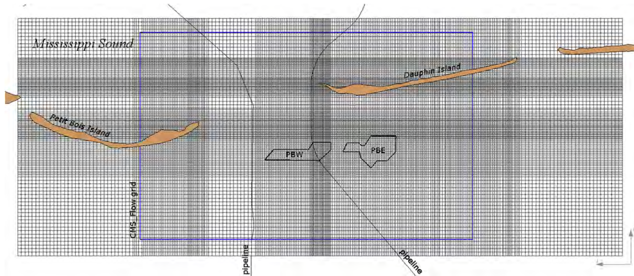
Figure 22. CMS-Wave fine nested grid mesh for Petit Bois Pass. The CMS-Flow mesh boundary is indicated using a blue box.
