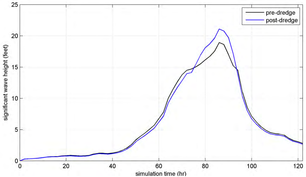
Figure 39. Plot of model wave height at the northern margin of PBE for existing and post-dredging conditions at the borrow site.
