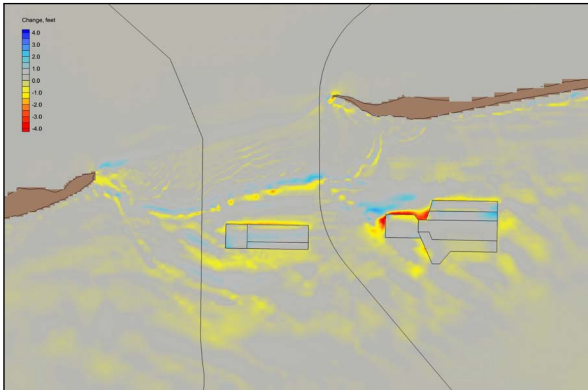
Figure 2: Morphological change for post-dredging conditions at the Petit Bois borrow sites from the simulation of Hurricane Katrina.
