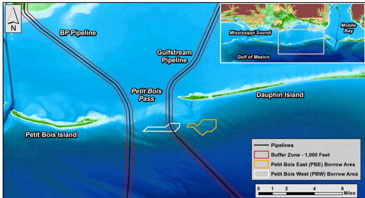
Figure 1. Project area illustrating borrow site locations relative to the Gulfstream pipeline.
