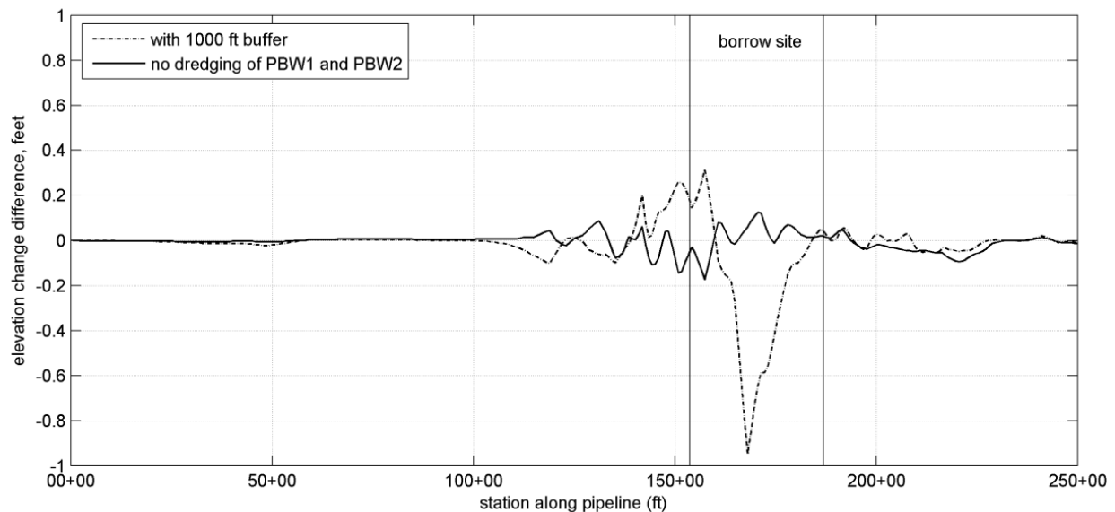
Figure 49. Comparison of bottom change difference (relative to existing conditions) between original PBW design with a 1000 ft pipeline buffer and the modified design with no dredging in PBW1 and PBW2 sub-sections.
