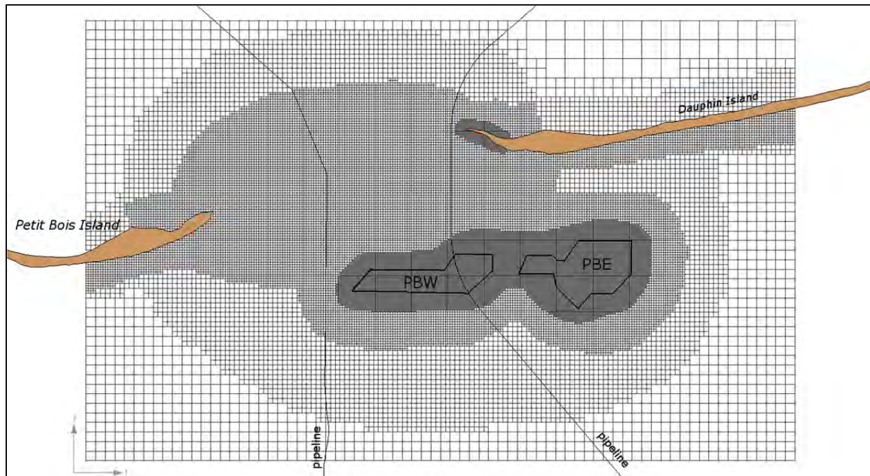
Figure 32. CMS-Flow telescoping mesh of Petit Bois Pass.
