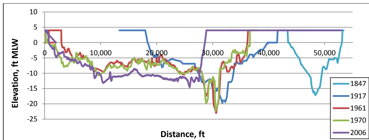
Figure 14. Historical inlet cross-sections for Petit Bois Pass illustrating changes in seafloor shape, 1847 to 2006.
