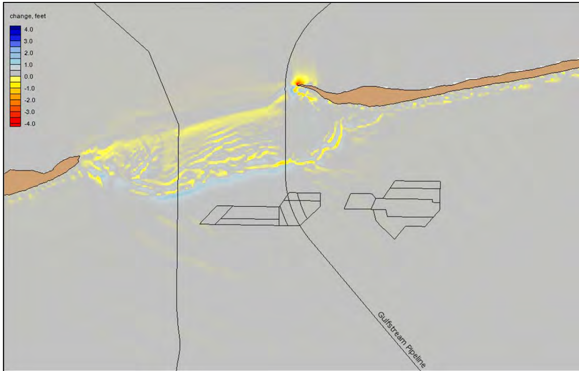
Figure 33. Morphological change computed for the month-long CMS simulation of February 1990.
