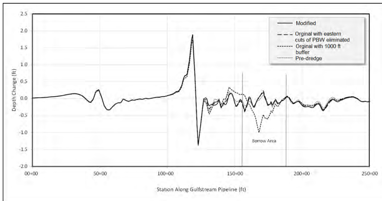
Figure 4: Comparison of change in depth along the Gulfstream pipeline as a result of the Hurricane Katrina model run for all geometries.
