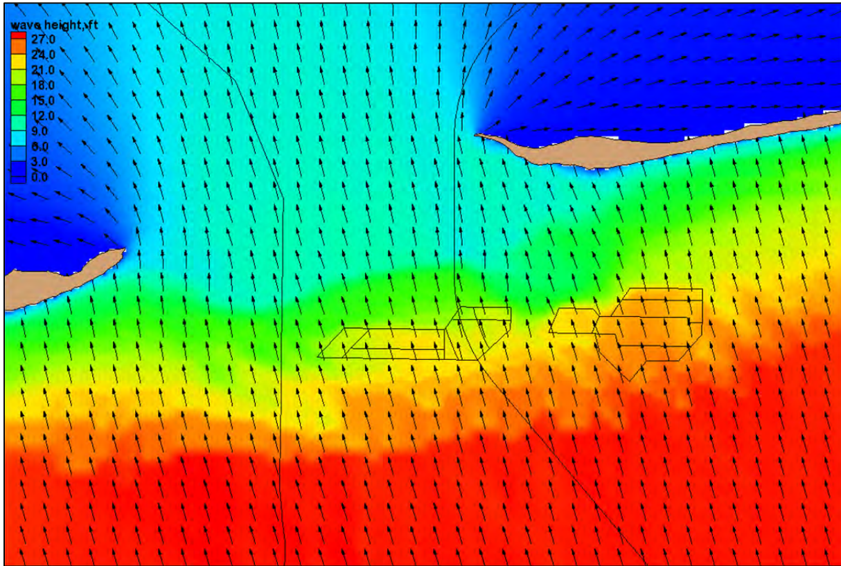
Figure 37. Contour plot of wave height with vectors that indicate wave direction for maximum wave height condition during Hurricane Katrina, for proposed dredged conditions (post-dredge) at the Petit Bois Borrow sites.
