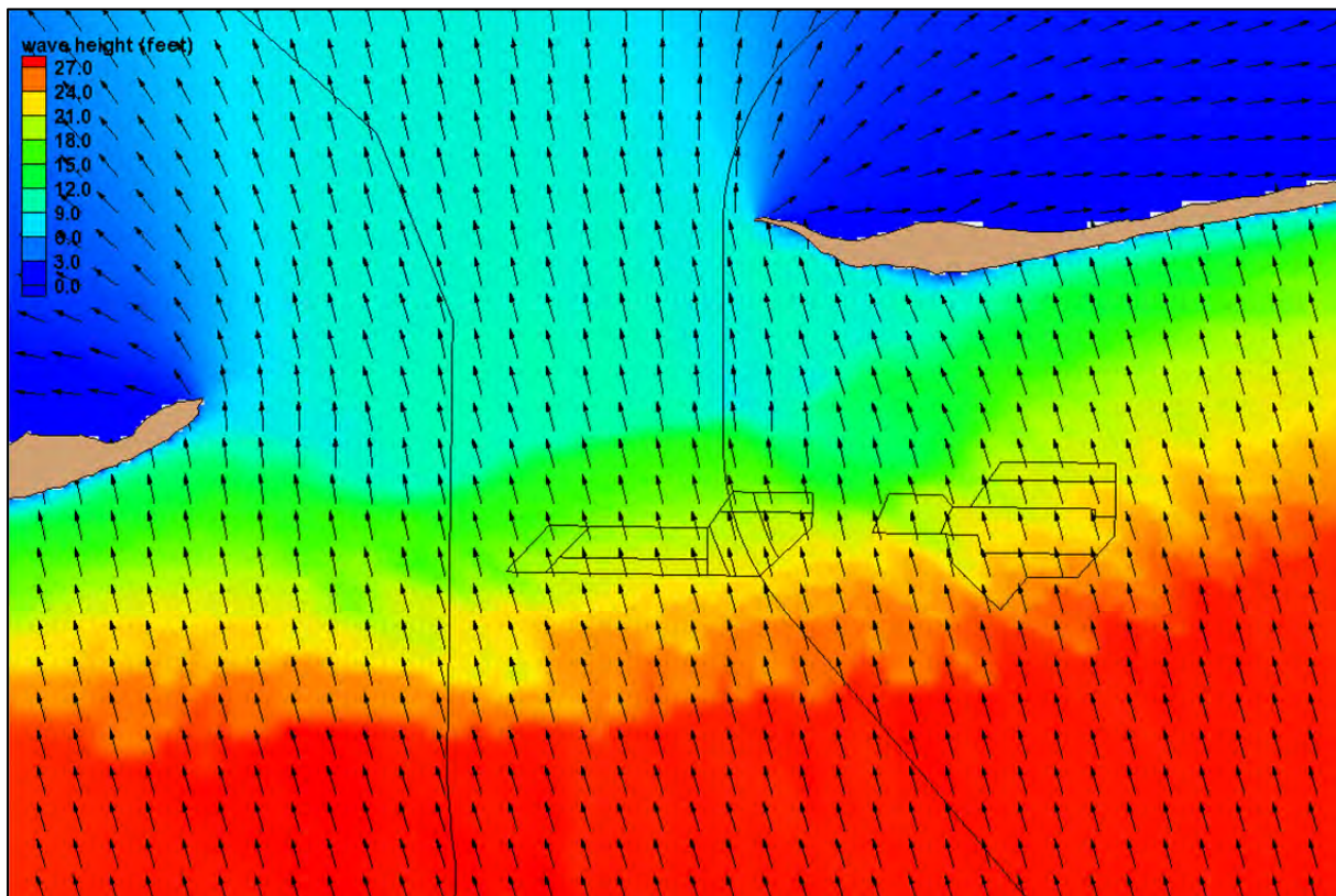
Figure 36. Contour plot of wave height with vectors indicating wave direction for maximum wave height conditions during Hurricane Katrina for existing conditions (pre-dredging) at the Petit Bois Pass.
