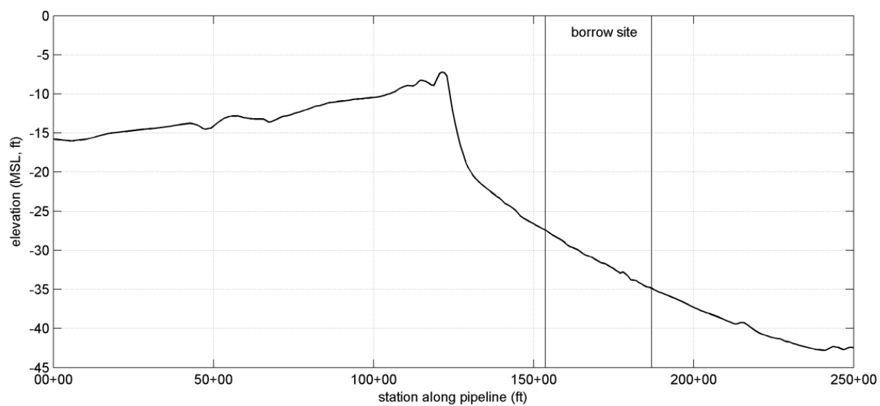
Figure 46. Bottom elevation along the Gulfstream pipeline transect (Figure 34), including the north and south limits of the PBW boundary.
