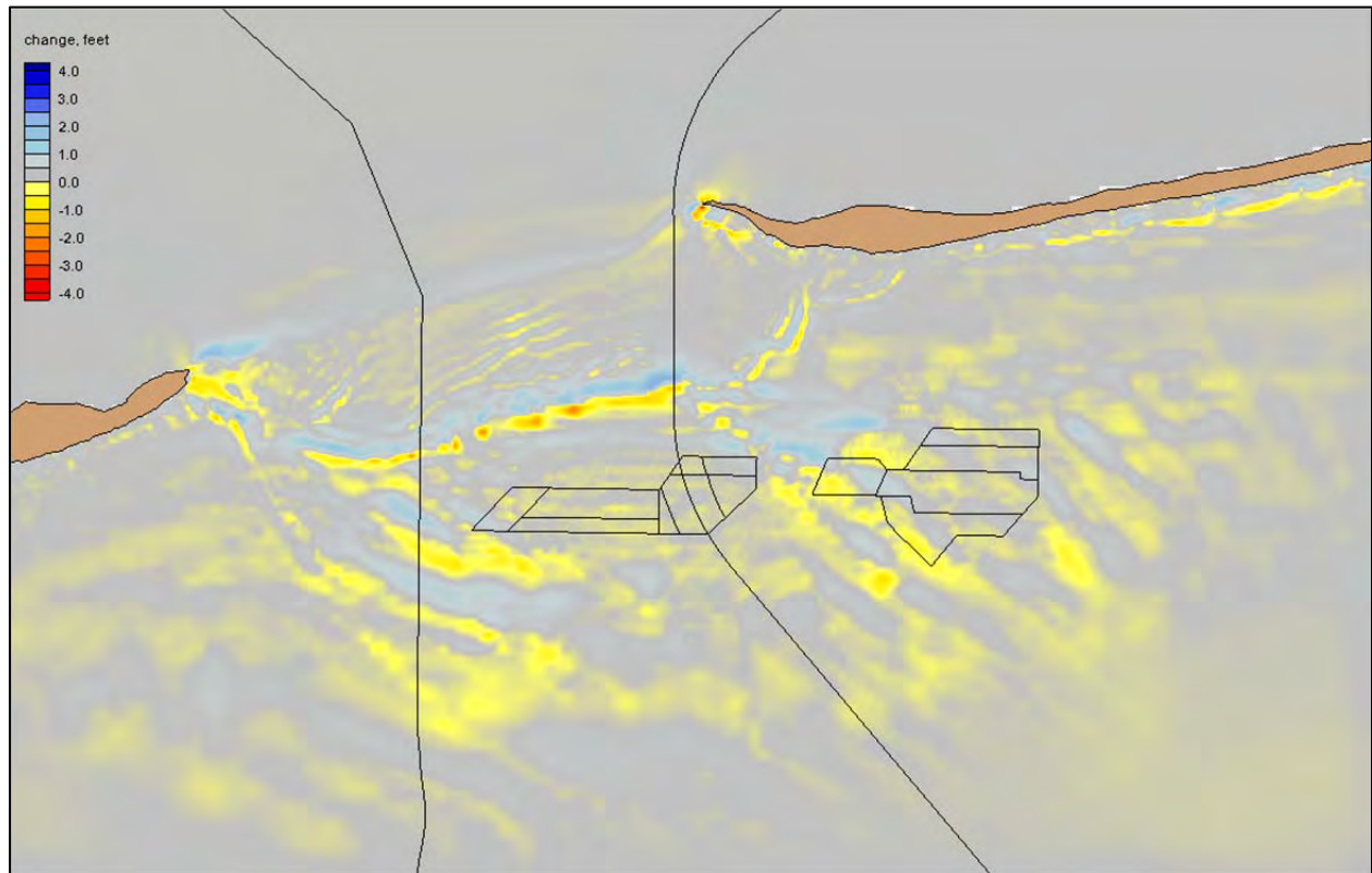
Figure 41. Contour map of bathymetric change for existing conditions at the Petit Bois borrow sites for the simulation of Hurricane Katrina. Borrow site boundaries and pipelines also are shown.
