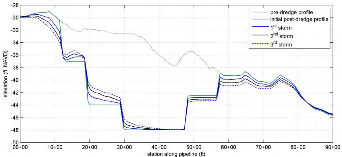
Figure 48. Bottom elevation along the PBE transect (Figure 34). Existing and post-dredging elevations are shown with bottom elevations after three consecutive runs of Hurricane Katrina.
