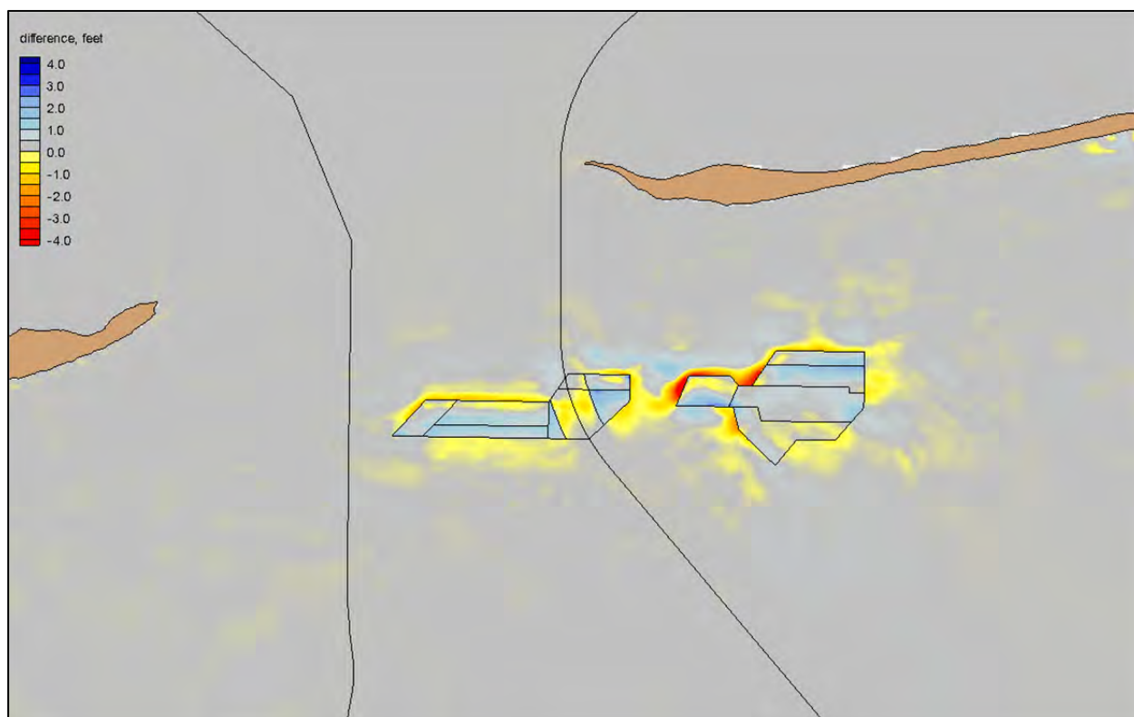
Figure 45. Difference map for existing and post-dredging morphology change from simulations of annual conditions.
