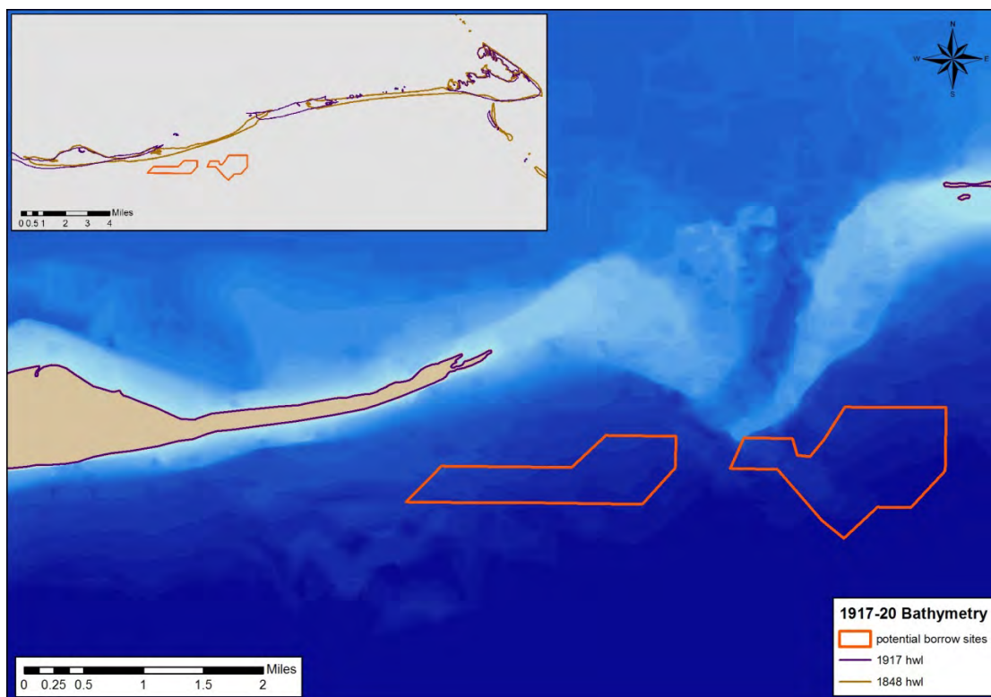
Figure 9. Bathymetric surface for Petit Bois Pass, 1917-20. Inset illustrates shoreline position prior to and after the hurricane of 1916.
