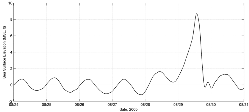
Figure 24. Water surface elevation offshore Petit Bois Pass during Hurricane Katrina from the Oceanweather storm hindcast.
