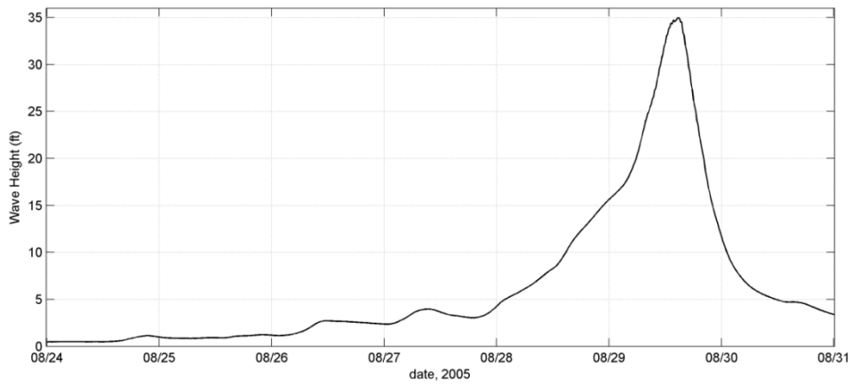
Figure 25. Significant wave height offshore Petit Bois Pass during Hurricane Katrina from the Oceanweather storm hindcast.
