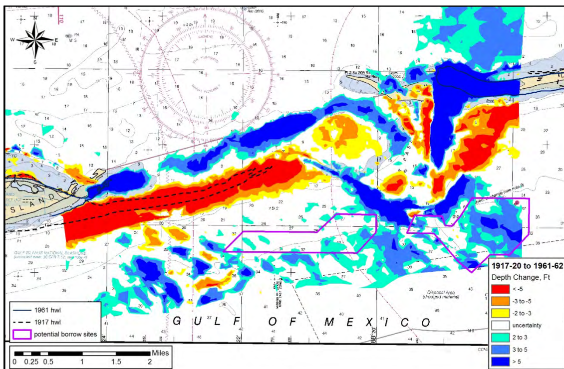
Figure 16. Bathymetric change between 1917-20 and 1961-62 for Petit Bois Pass.
