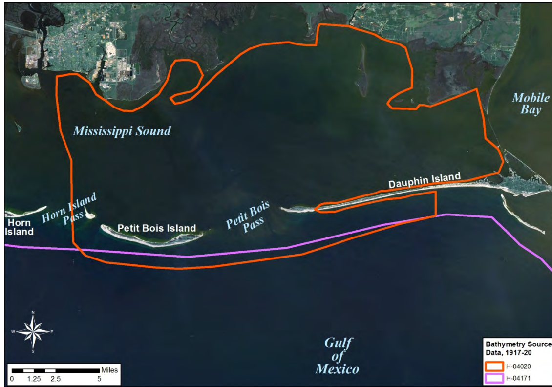
Figure 3. Hydrographic survey coverage, 1917-20.
