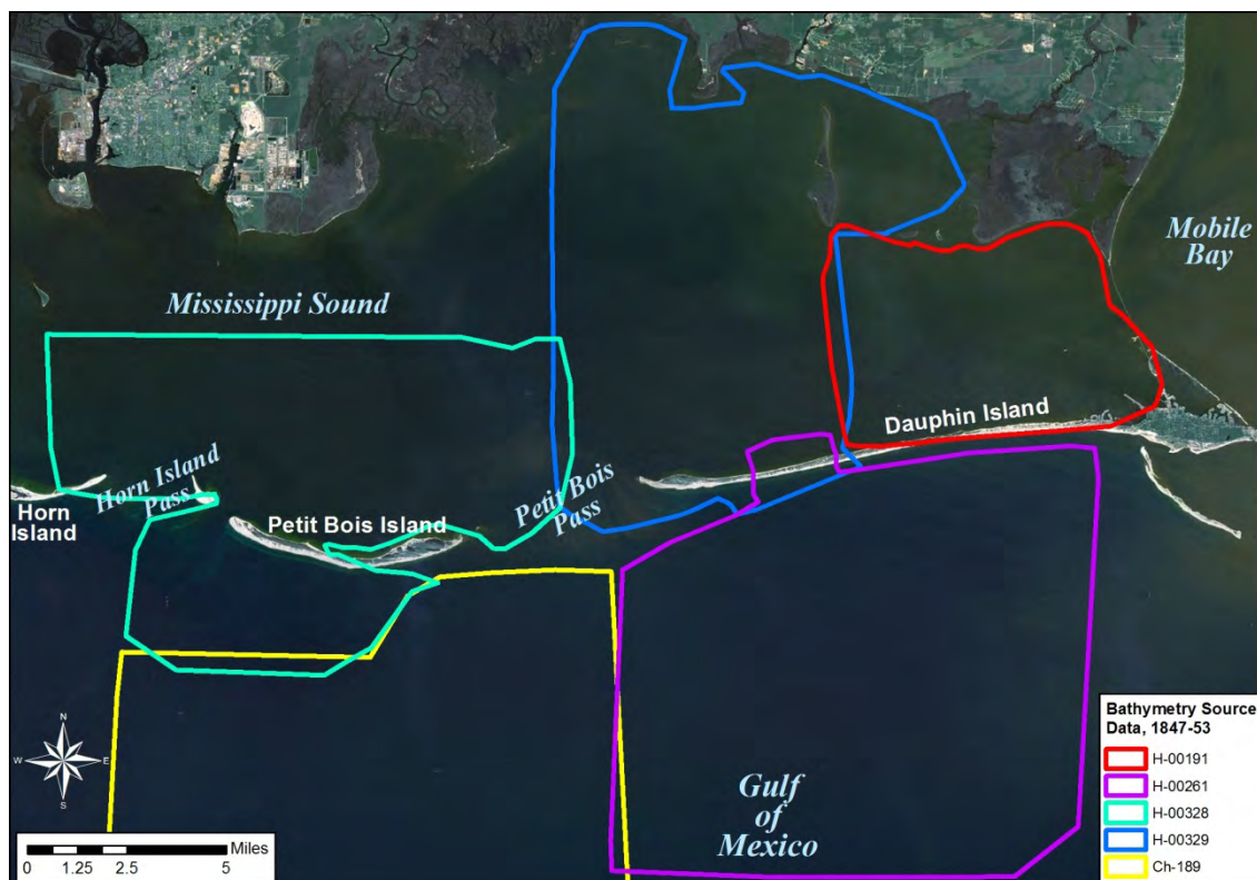
Figure 2. Hydrographic survey coverage, 1847-53.
