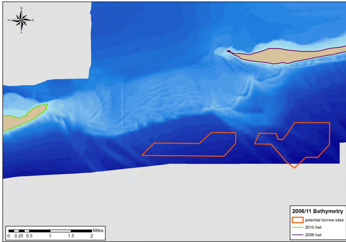
Figure 12. Bathymetric surface for Petit Bois Pass, 2006/11.
