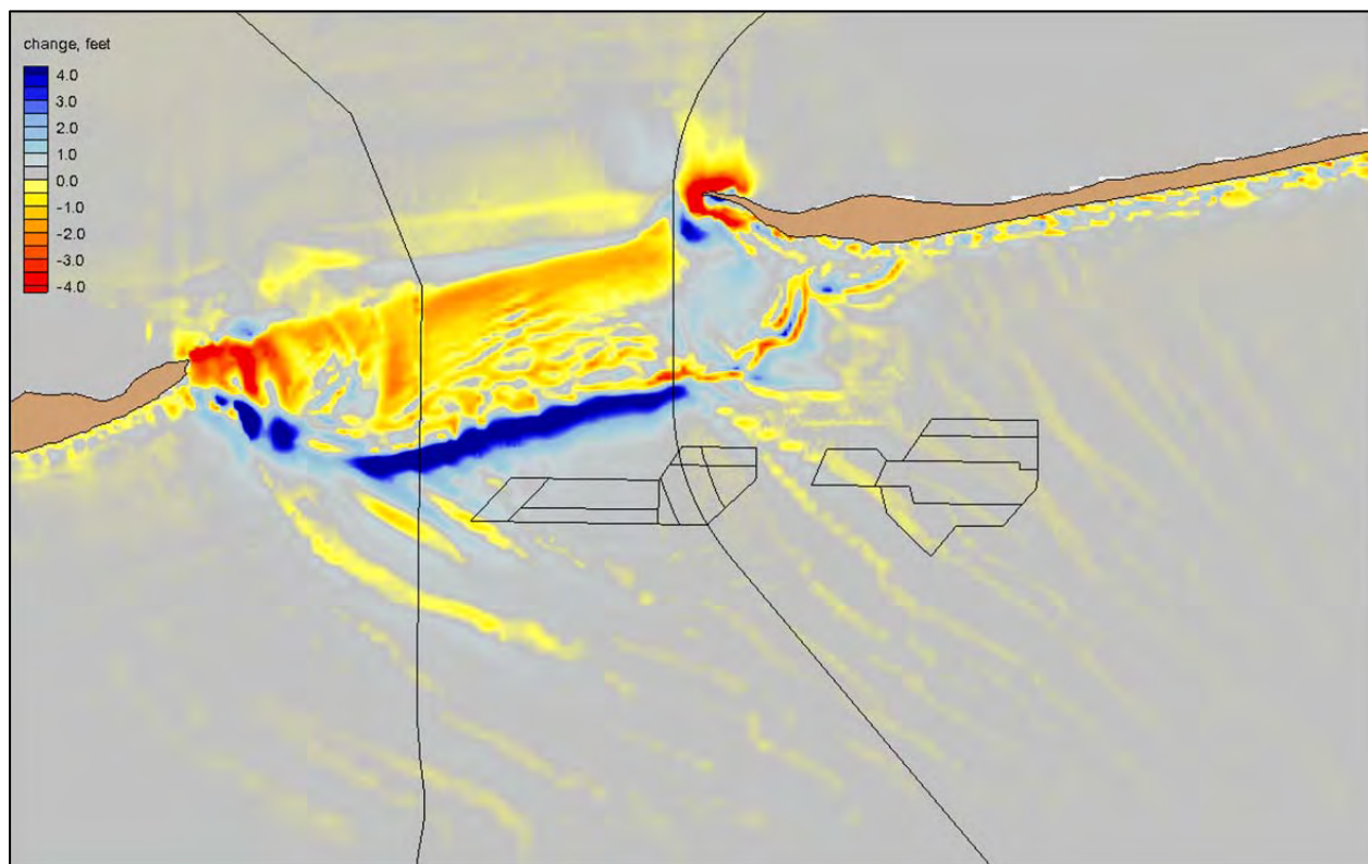
Figure 40. Contour map of bathymetric change for existing conditions at the Petit Bois borrow sites, from the year-long simulation. Borrow site boundaries and pipelines also are shown.
