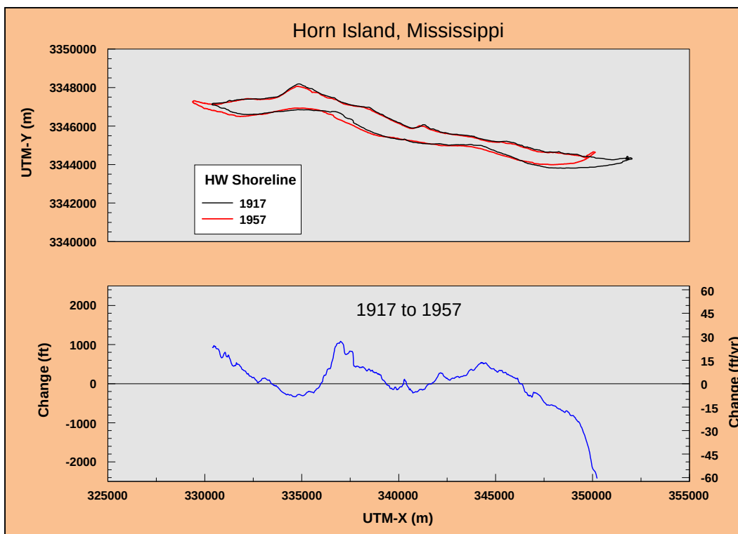
Figure C19. Change in historical shoreline position, Horn Island, MS, 1917 to 1957.
