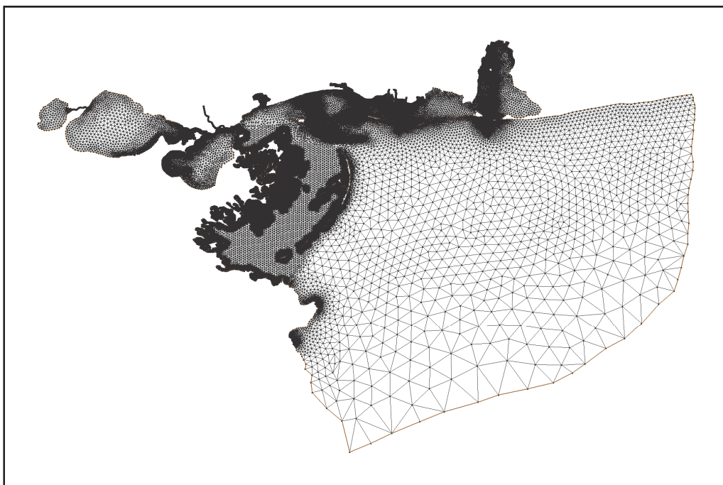
Figure 3-1. ADCIRC grid.
