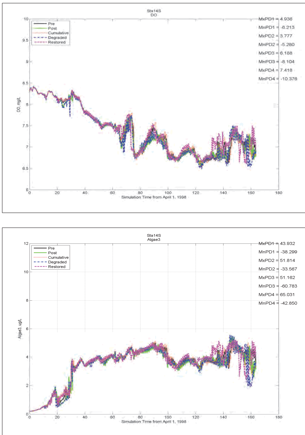
Figure E-71. Comparison of DO, Chlorophyll, and Salinity at Station 14 (Figure 5-8) for results from simulations representing Pre, Post, Restored, Degraded, and Cumulative conditions (continued).
