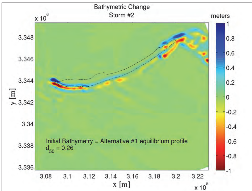
Figure G-34. Alternative #1 Restored conditions for Storm #2; Template B; Without borrow pits.
