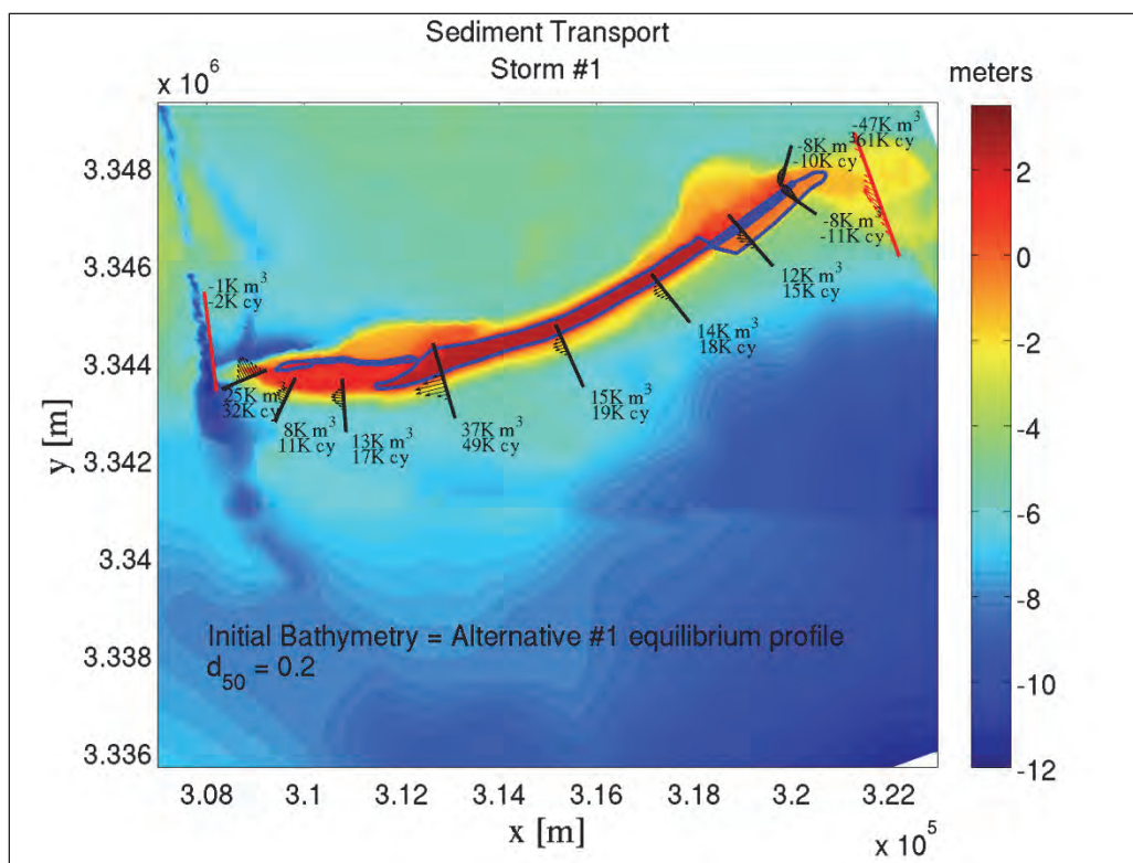
Figure G-5. Alternative #1 Restored conditions for Storm #1; Template A; Without borrow pits.
