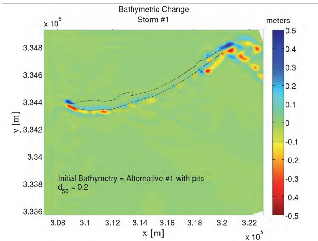
Figure G-23. Alternative #1 Restored conditions for Storm #1; Template A; With borrow pits.
