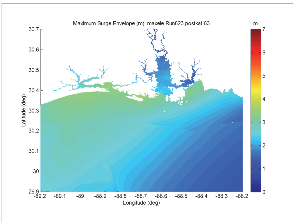
Figure F-41. Maximum surge envelope for Storm 823, Post-Katrina condition.
