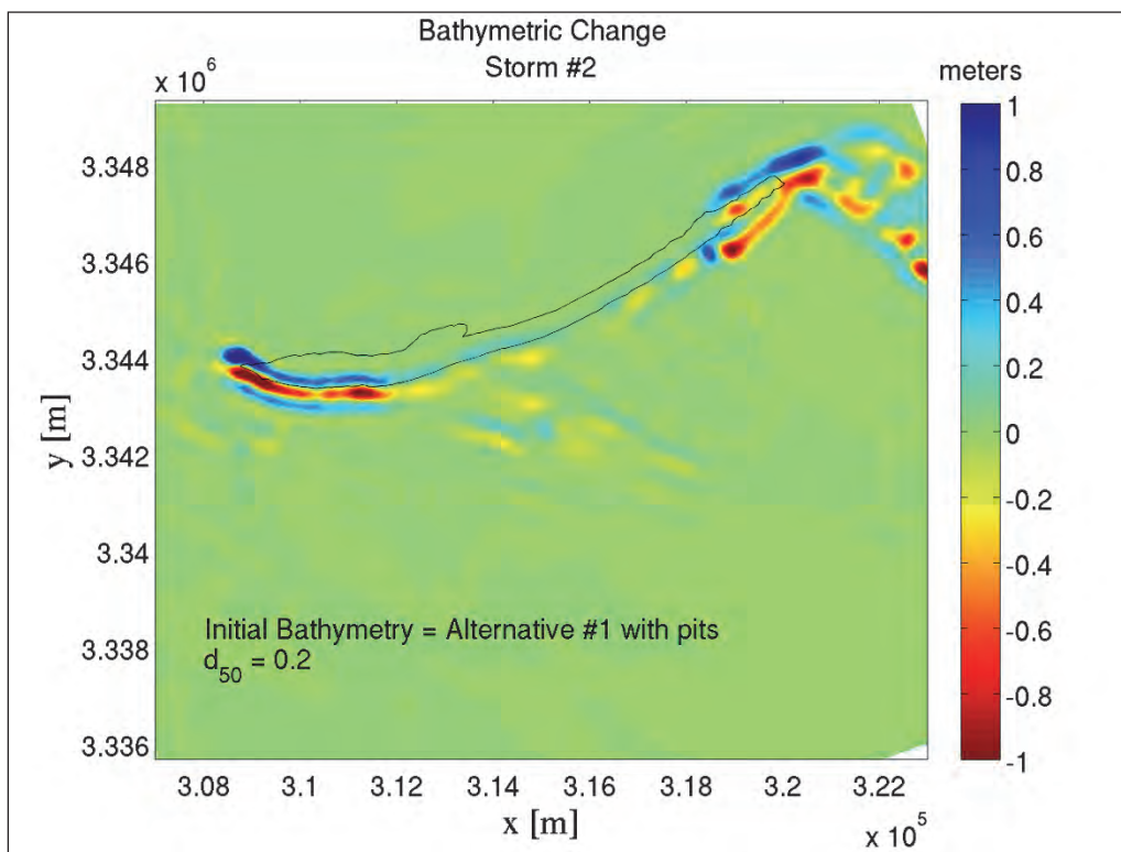
Figure G-30. Alternative #1 Restored conditions for Storm #2; Template A; With borrow pits.
