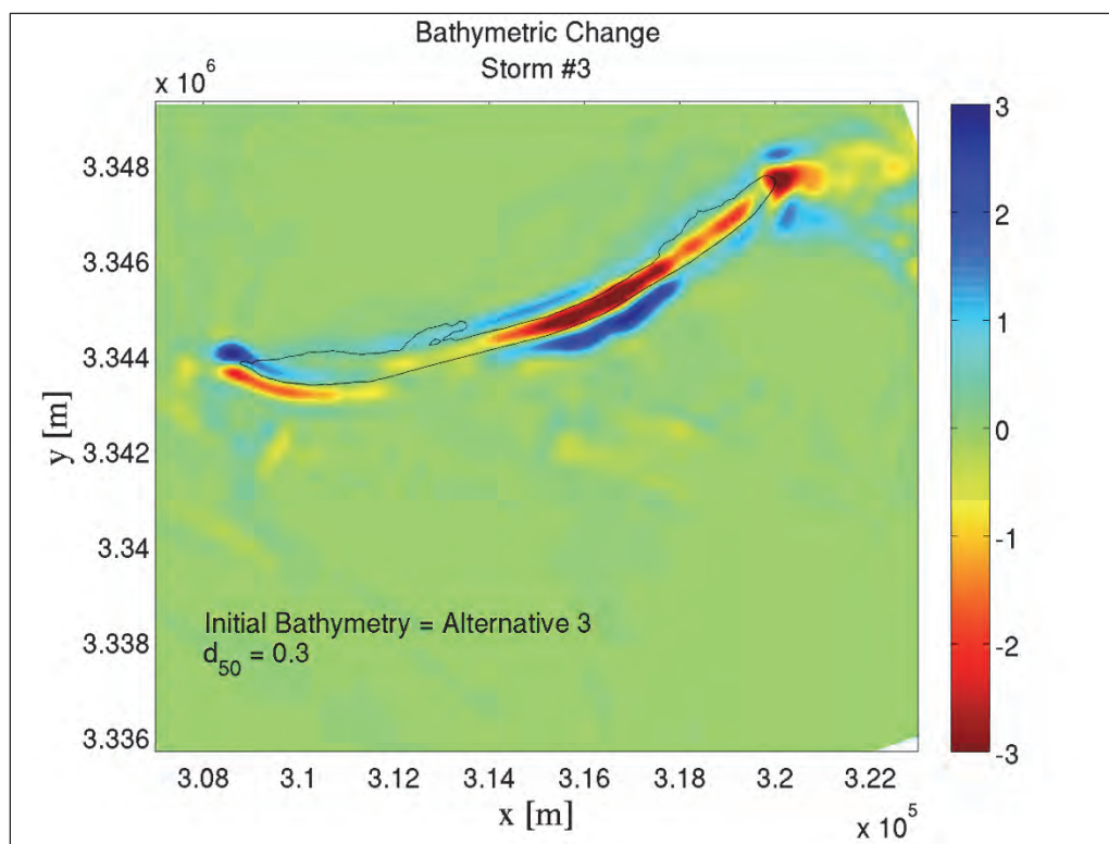
Figure J-12. Alternative 3 Restored conditions for Storm #3; d_{50} = 0.30 mm; With borrow pit.
