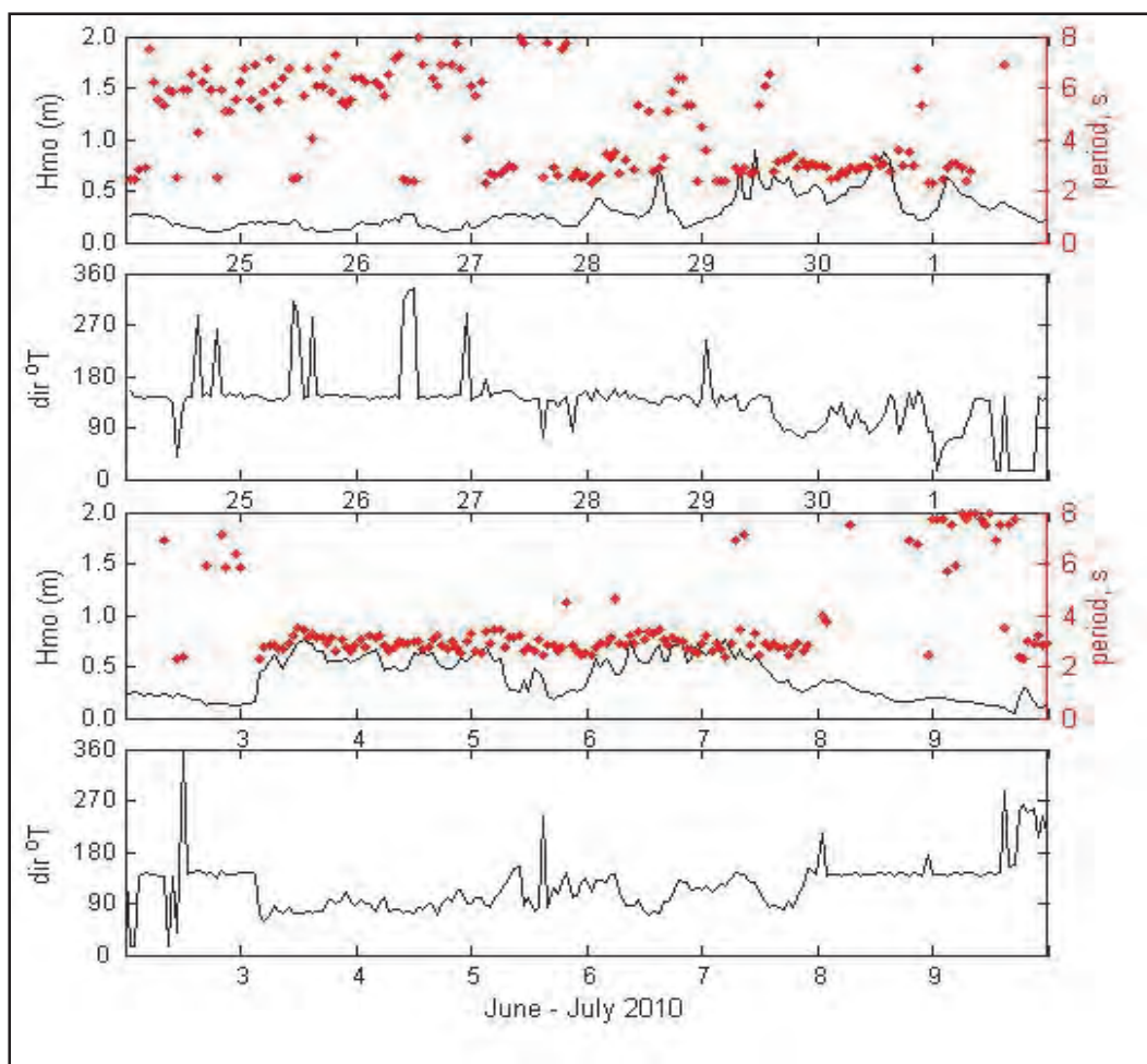
Figure A-12. Wave direction (direction waves are coming from at the spectral peak), H_{mo} , and wave period (at the spectral peak), for the gauge in the Mississippi Sound from June 24 through July 9, 2010.
