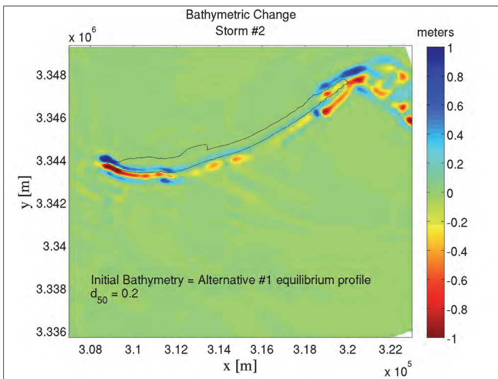
Figure G-33. Alternative #1 Restored conditions for Storm #2; Template A; Without borrow pits.
