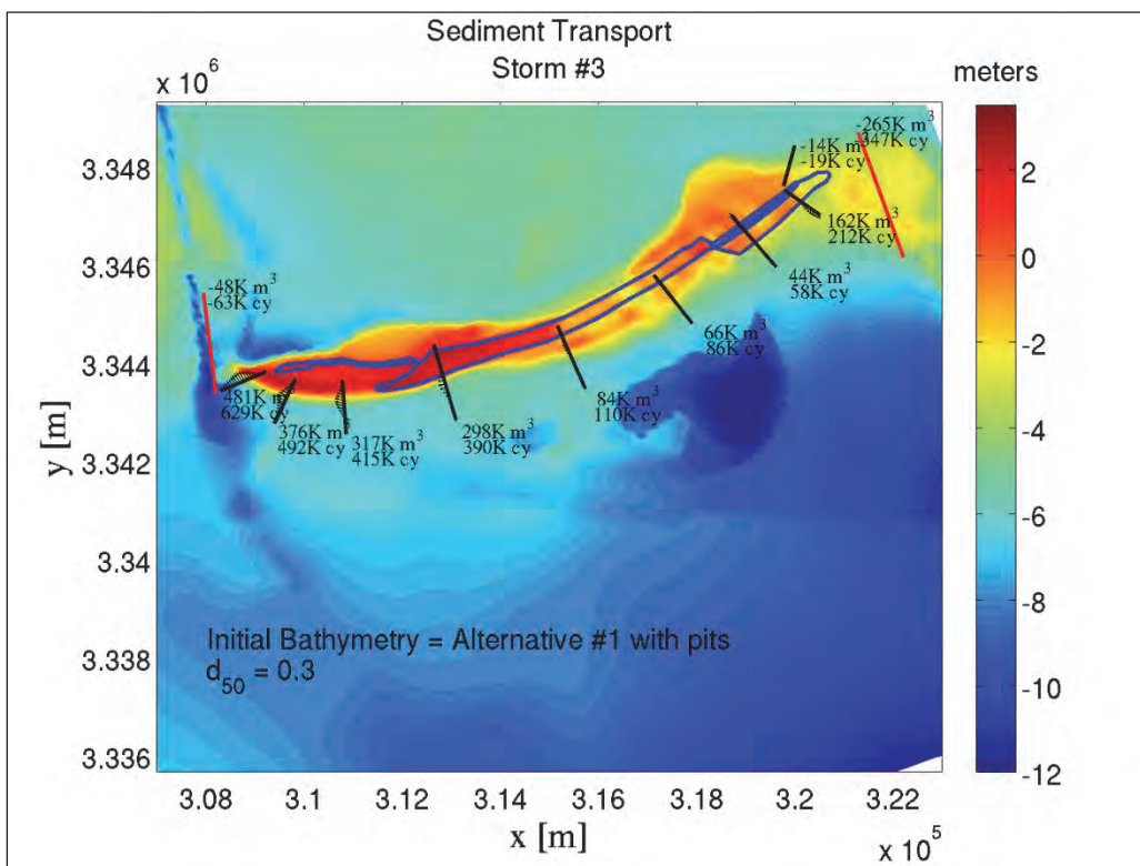
Figure G-18. Alternative #1 Restored conditions for Storm #3; Template C; With borrow pits.
