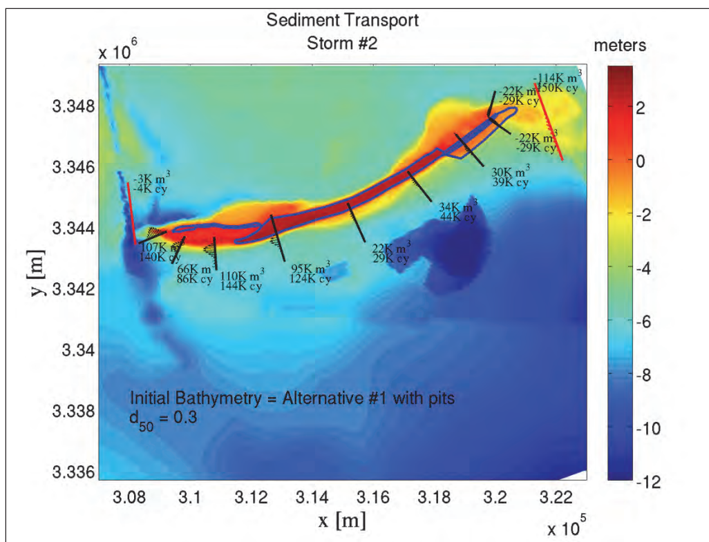
Figure G-11. Alternative #1 Restored conditions for Storm #2; Template C; With borrow pits.
