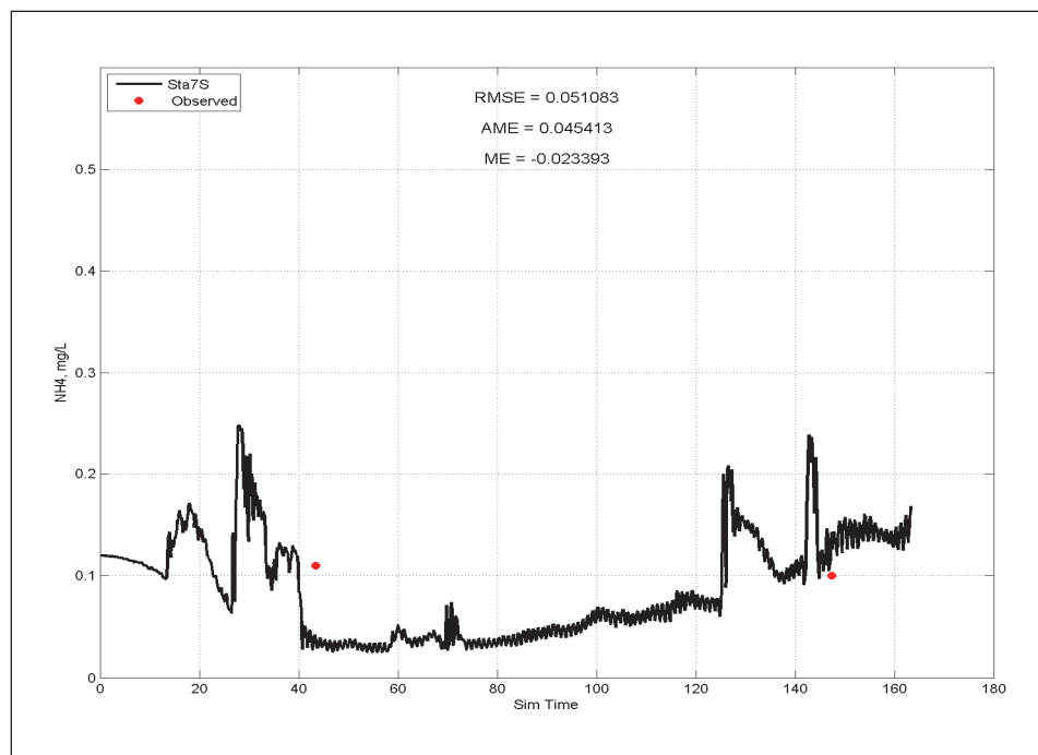
Figure E-40. Calibration results for \text{NH}_4 at Station 7 for surface layer (upper) and bottom layer (lower).
