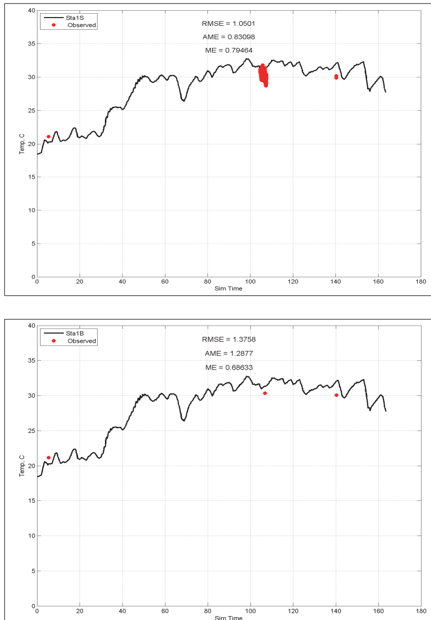
Figure E-1. Calibration results for temperature at Station 1 for surface layer (upper) and bottom layer (lower).
