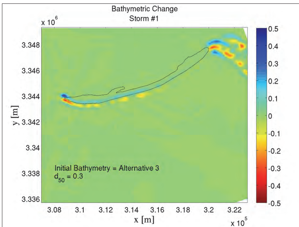
Figure J-8. Alternative 3 Restored conditions for Storm #1; d_{50} = 0.30 mm; With borrow pit.
