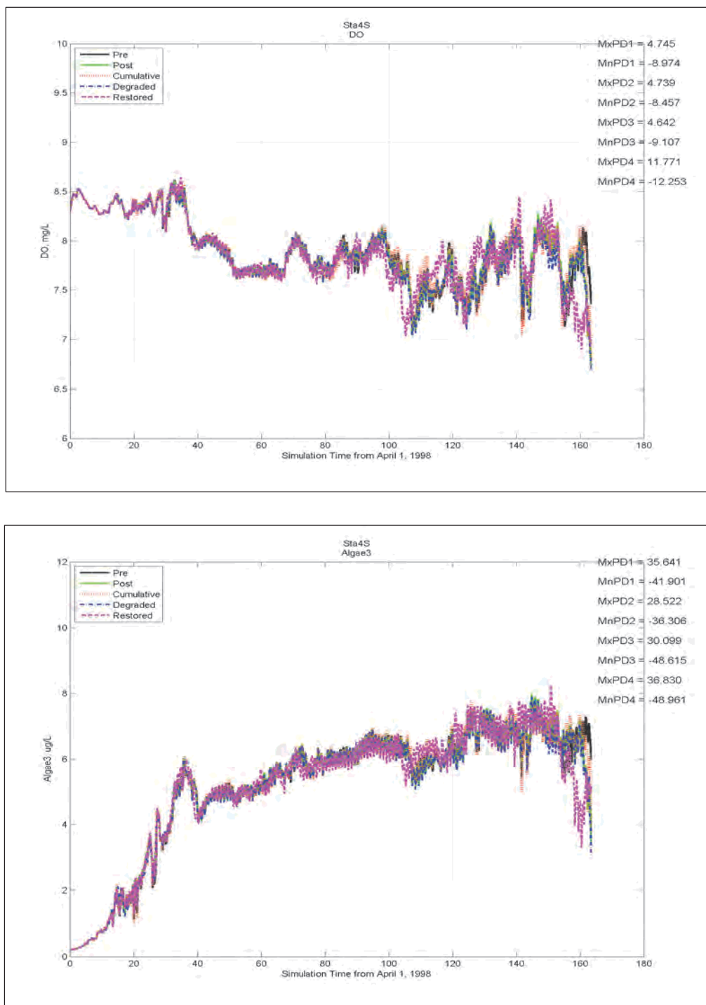
Figure E-63. Comparison of DO, Chlorophyll, and Salinity at Station 4 (Figure 5-2) for results from simulations representing Pre, Post, Restored, Degraded, and Cumulative conditions (continued).
