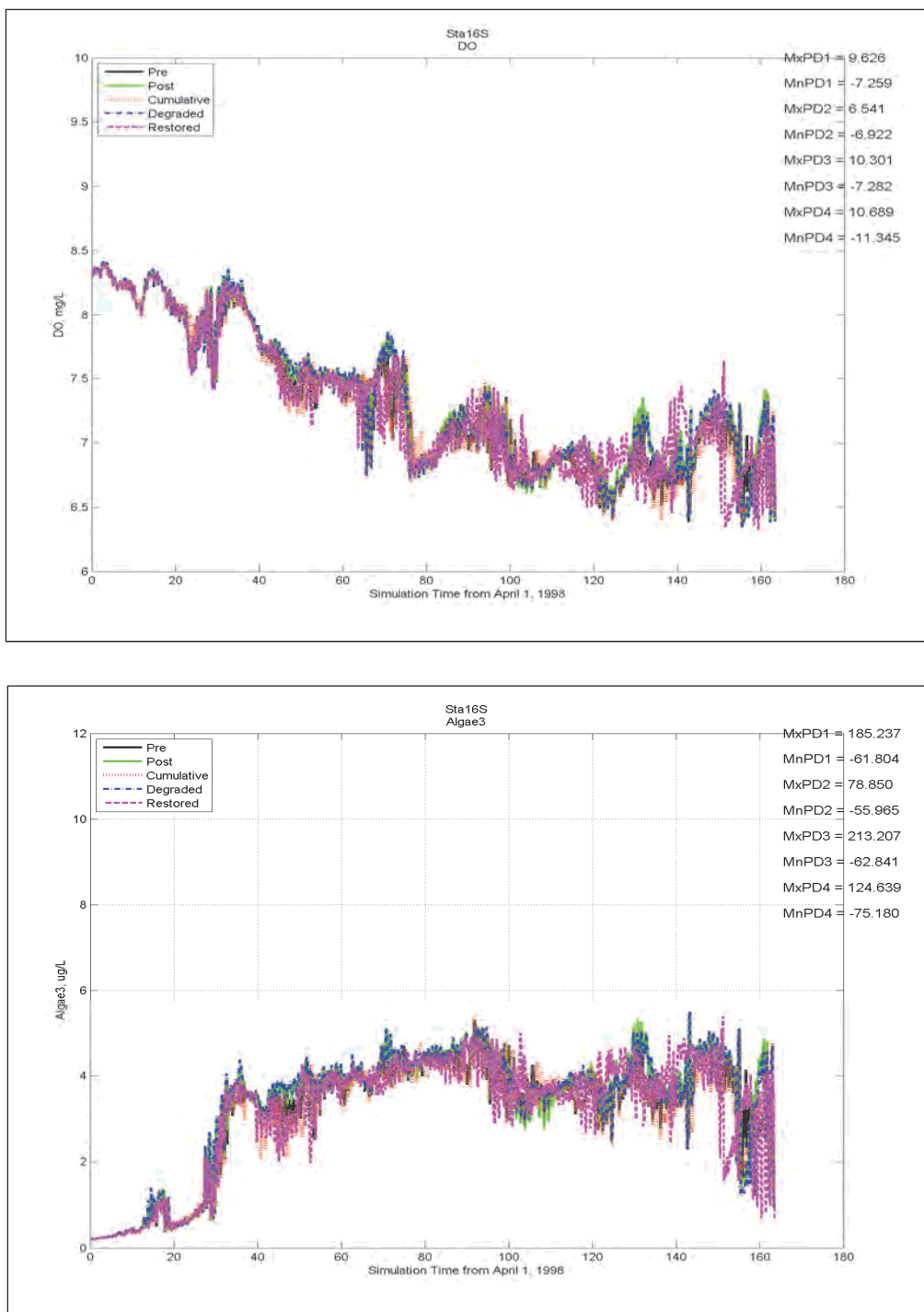
Figure E-73. Comparison of DO, Chlorophyll, and Salinity at Station 16 (Figure 5-8) for results from simulations representing Pre, Post, Restored, Degraded, and Cumulative conditions (continued).
