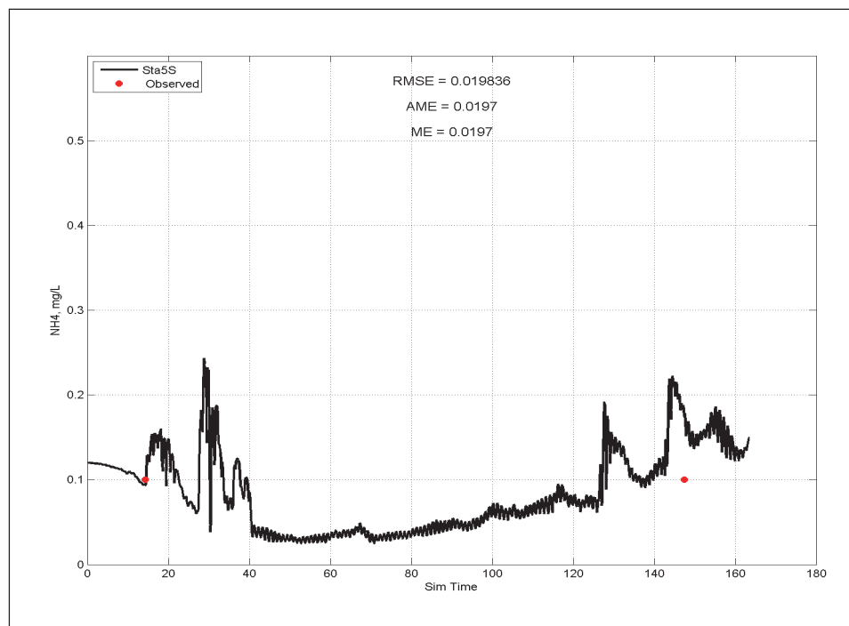
Figure E-28. Calibration results for \text{NH}_4 at Station 5 for surface layer (upper) and bottom layer (lower).
