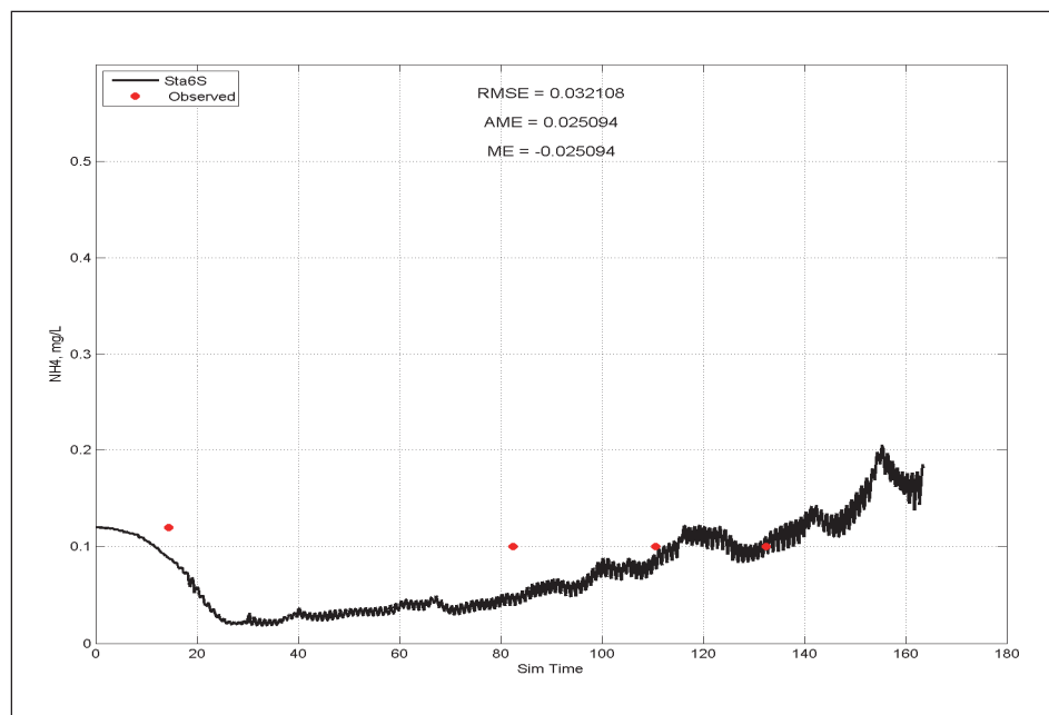
Figure E-34. Calibration results for \text{NH}_4 at Station 6 for surface layer (upper) and bottom layer (lower).
