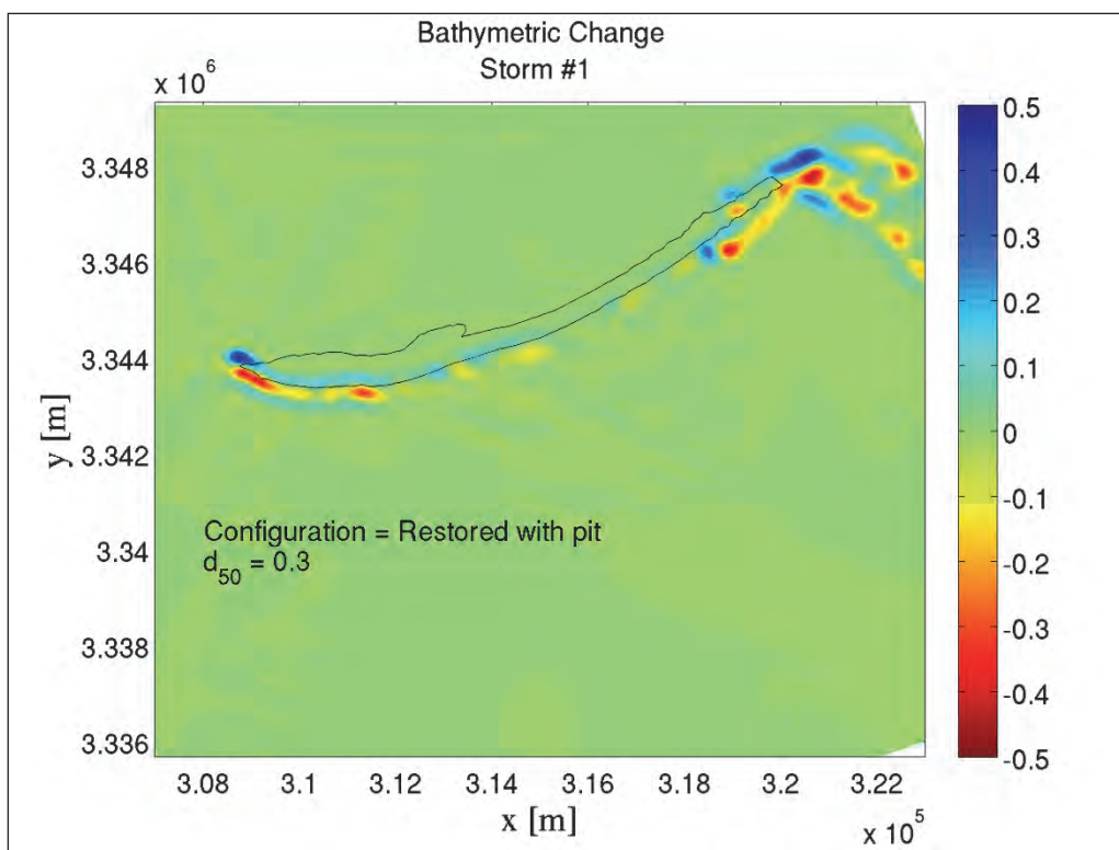
Figure H-4. Restored conditions for Storm #1; d_{50} = 0.30 mm (Template #3); With borrow pits.
