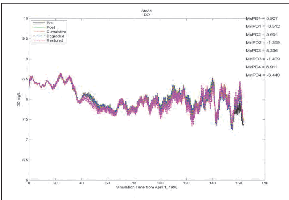
Figure E-66. Comparison of DO, Chlorophyll, and Salinity at Station 8 (Figure 5-2) for results from simulations representing Pre, Post, Restored, Degraded, and Cumulative conditions (continued).
