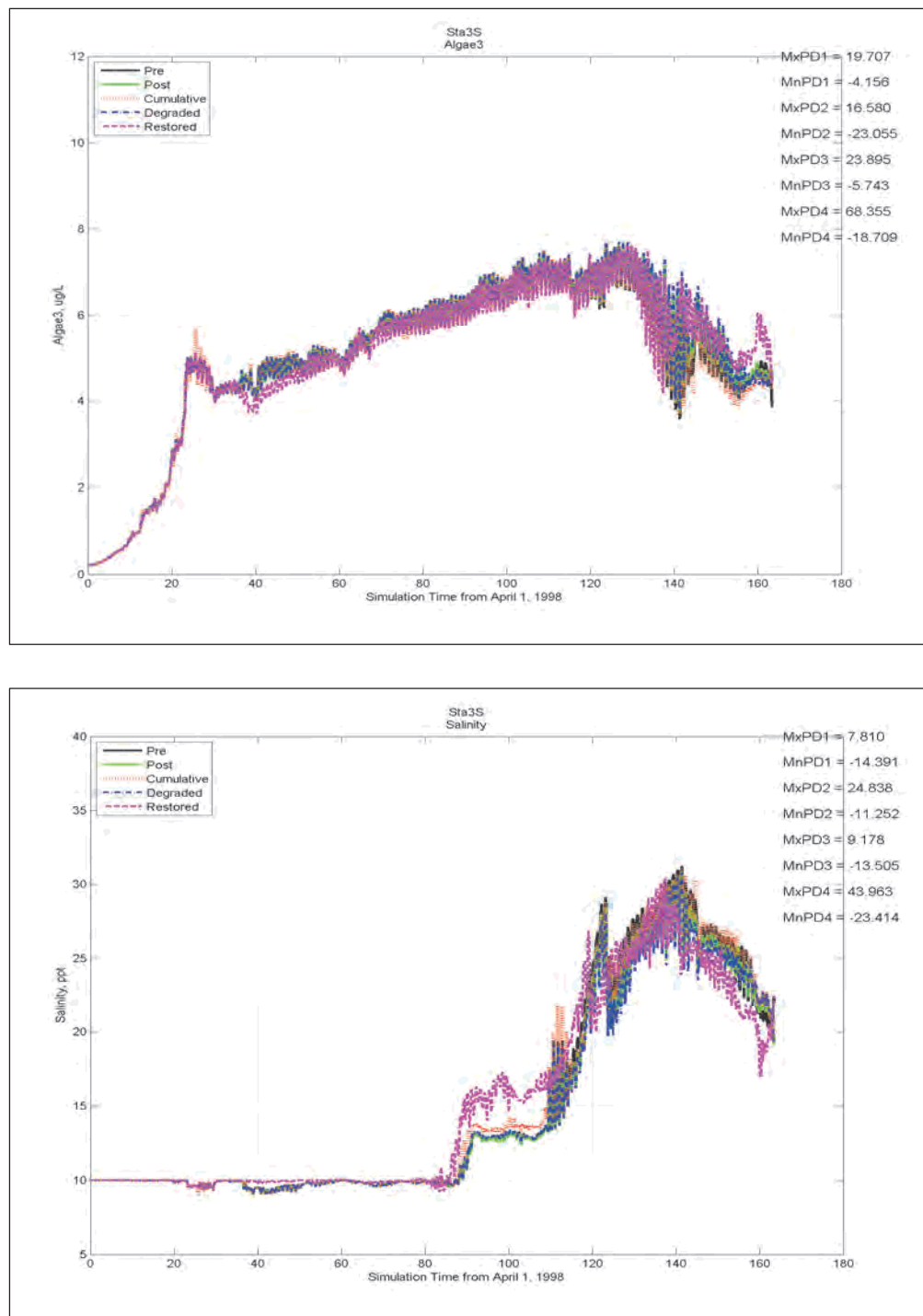
Figure E-62. Concluded.
