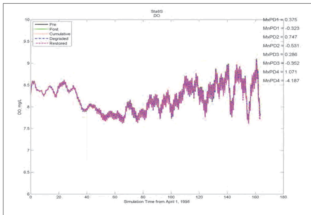
Figure E-64. Comparison of DO, Chlorophyll, and Salinity at Station 6 (Figure 5-2) for results from simulations representing Pre, Post, Restored, Degraded, and Cumulative conditions (continued).
