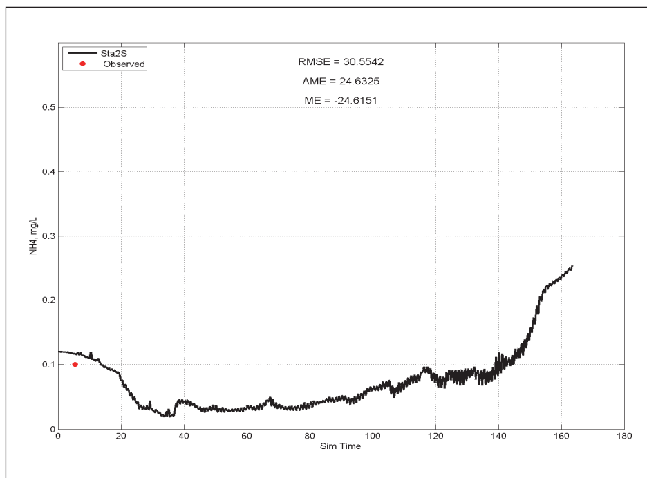
Figure E-10. Calibration results for \text{NH}_4 at Station 2 for surface layer (upper) and bottom layer (lower).
