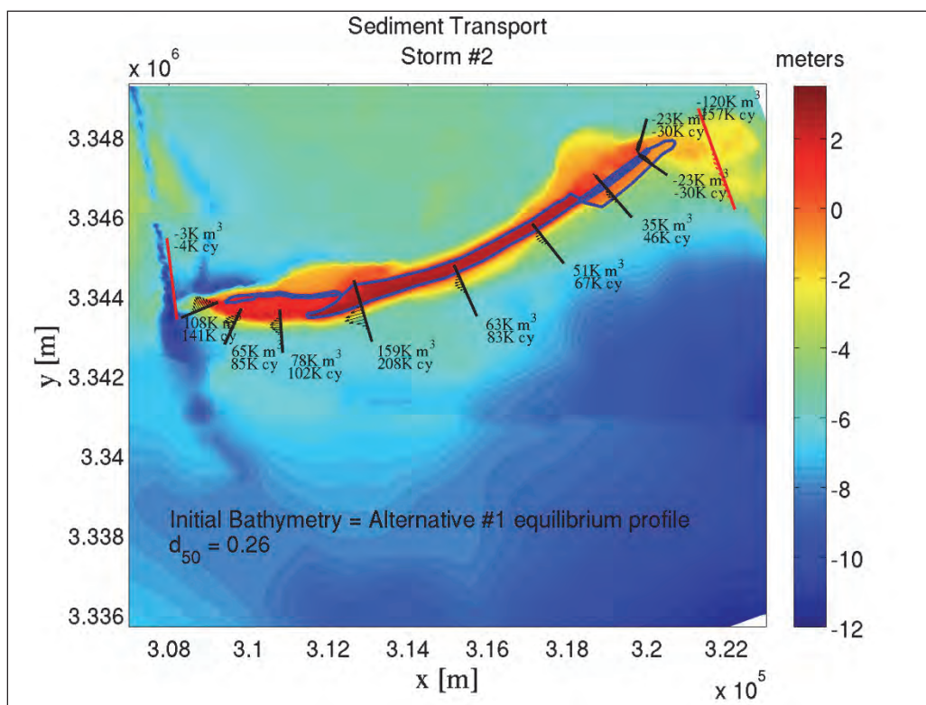
Figure G-13. Alternative #1 Restored conditions for Storm #2; Template B; Without borrow pits.
