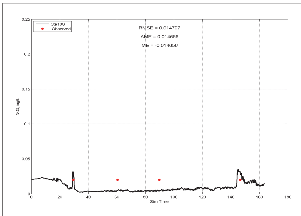
Figure E-59. Calibration results for \text{NO}_3 at Station 10 for surface layer (upper) and bottom layer (lower).
