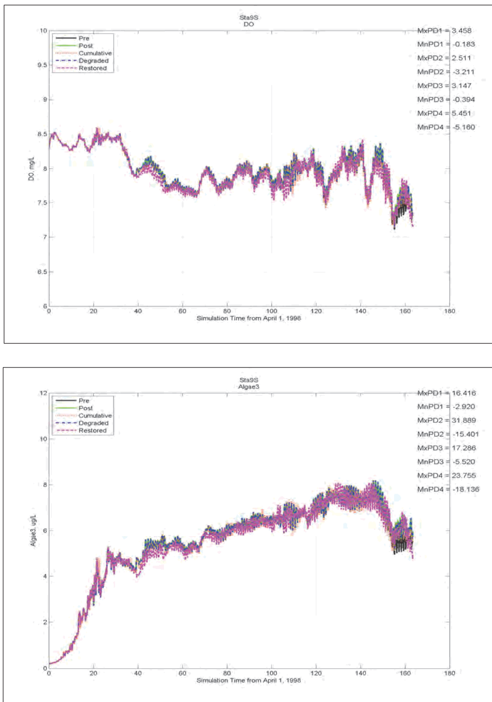
Figure E-67. Comparison of DO, Chlororophyll, and Salinity at Station 9 (Figure 5-2) for results from simulations representing Pre, Post, Restored, Degraded, and Cumulative conditions (continued).
