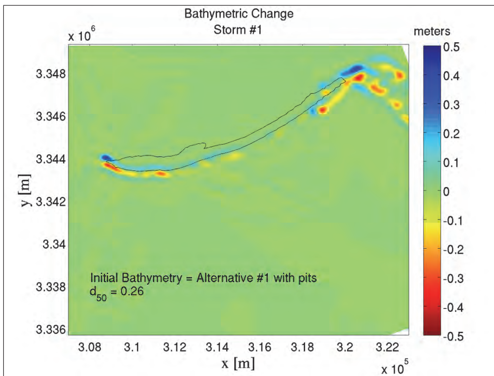
Figure G-24. Alternative #1 Restored conditions for Storm #1; Template B; With borrow pits.
