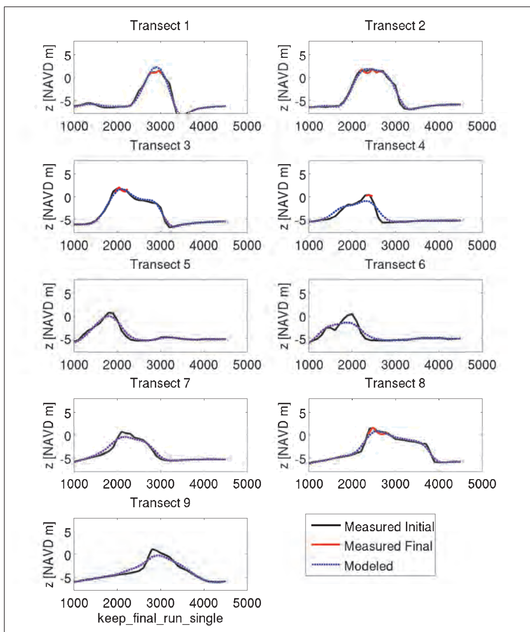
Figure 7-25. Initial and final profile transects for the Hurricane Katrina validation. Note: Transects are shown in Figures 7-20, 7-21, and 7-23 and are numbered 1-9 beginning with #1 on the west side.
