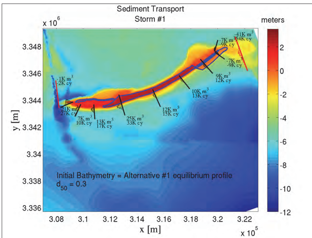
Figure G-7. Alternative #1 Restored conditions for Storm #1; Template C; Without borrow pits.
