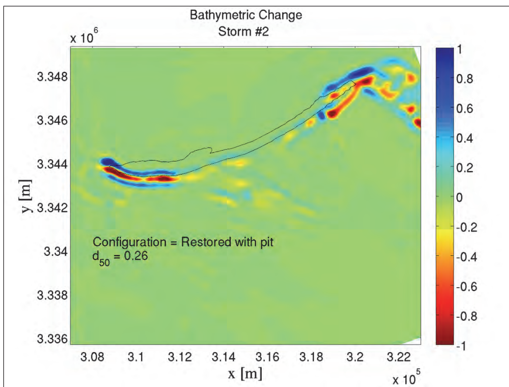
Figure H-10. Restored conditions for Storm #2; d_{50} = 0.26 mm (Template #2); With borrow pits.
