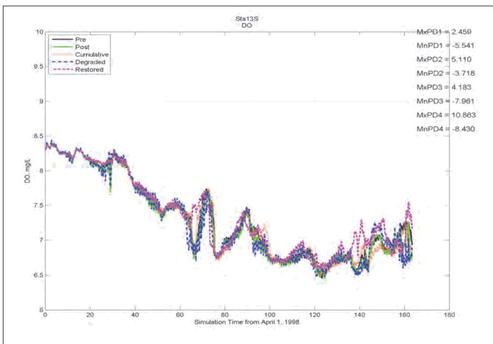
Figure E-70. Comparison of DO, Chlorophyll, and Salinity at Station 13 (Figure 5-8) for results from simulations representing Pre, Post, Restored, Degraded, and Cumulative conditions (continued).
