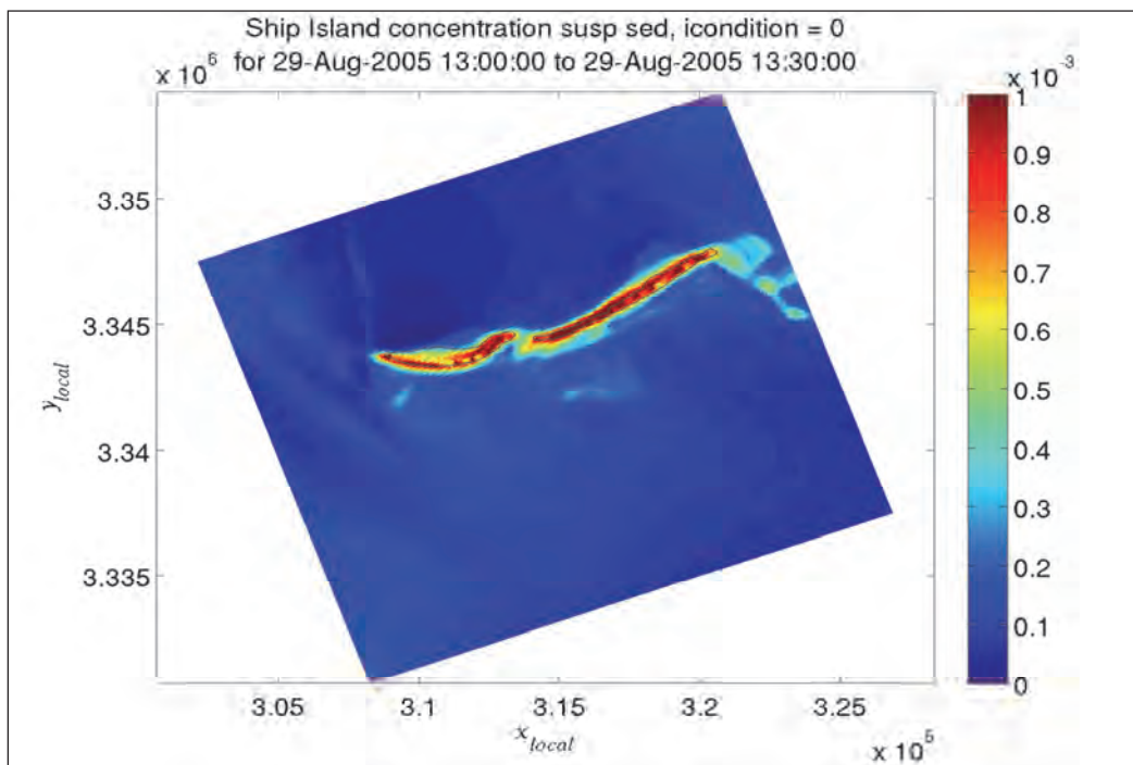
Figure 7-17. Volumetric concentration of suspended sediment modeled during the peak of Hurricane Katrina. Note: The largest concentrations are in excess of 0.1 percent [ \text{m}^3/\text{m}^3 ].
