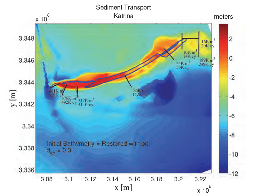
Figure I-4. Restored conditions for Katrina; d_{50} = 0.30 mm (Template #3); With borrow pits.
