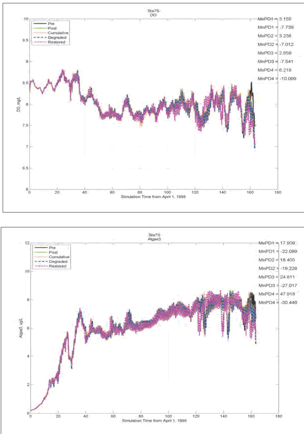
Figure E-65. Comparison of DO, Chlorophyll, and Salinity at Station 7 (Figure 5-2) for results from simulations representing Pre, Post, Restored, Degraded, and Cumulative conditions (continued).
