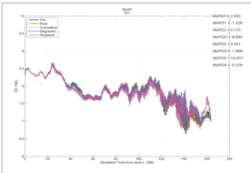
Figure E-62. Comparison of DO, Chlororphyll, and Salinity at Station 3 (Figure 5-2) for results from simulations representing Pre, Post, Restored, Degraded, and Cumulative conditions (continued).
