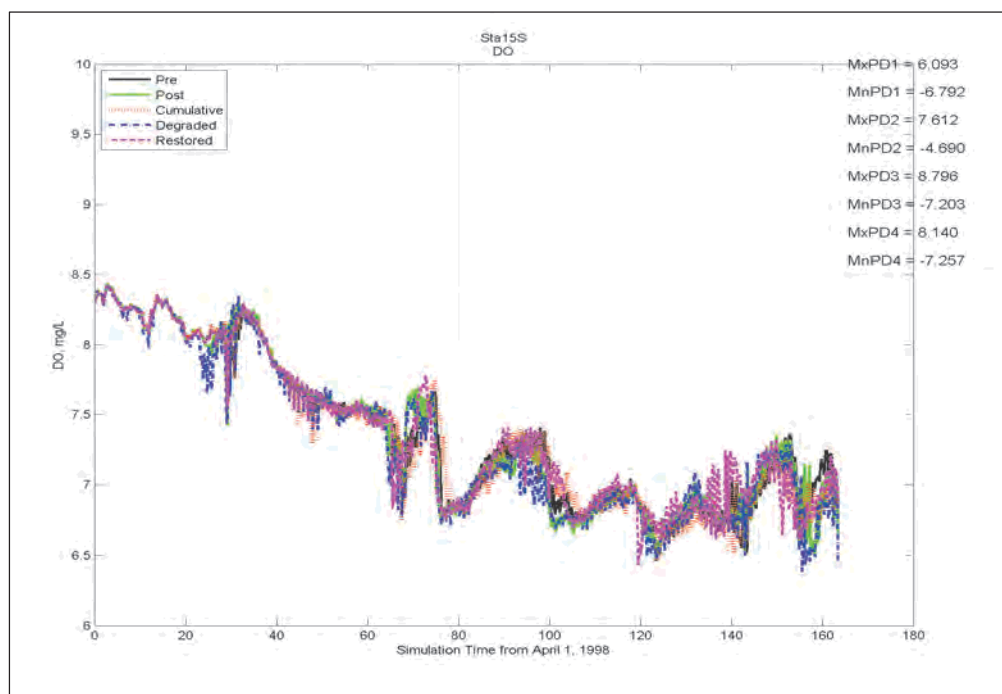
Figure E-72. Comparison of DO, Chlorophyll, and Salinity at Station 15 (Figure 5-8) for results from simulations representing Pre, Post, Restored, Degraded, and Cumulative conditions (continued).
