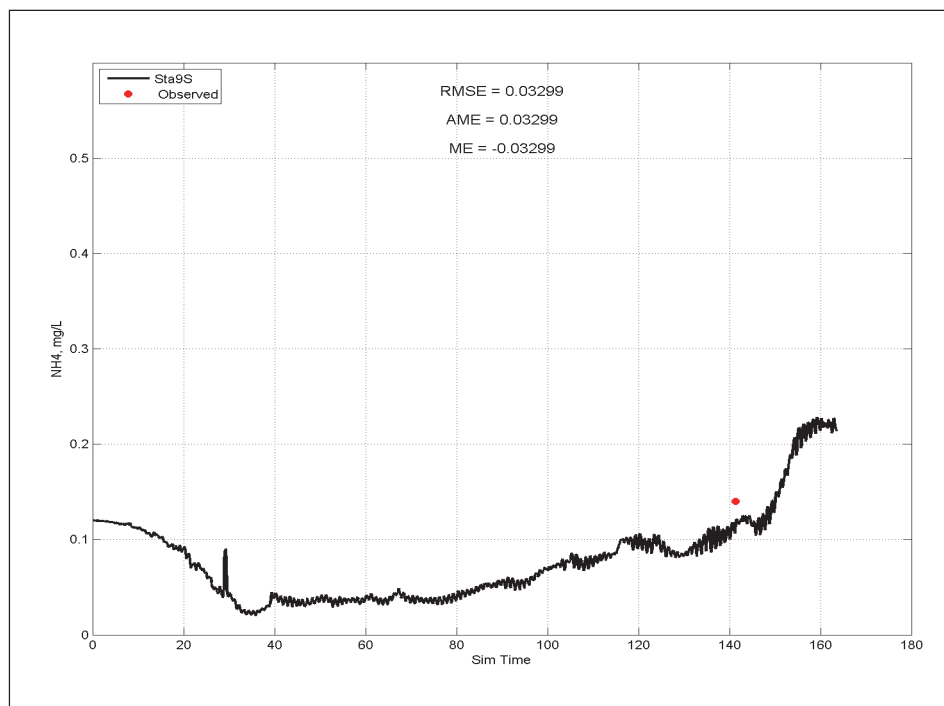
Figure E-52. Calibration results for \text{NH}_4 at Station 9 for surface layer (upper) and bottom layer (lower).
