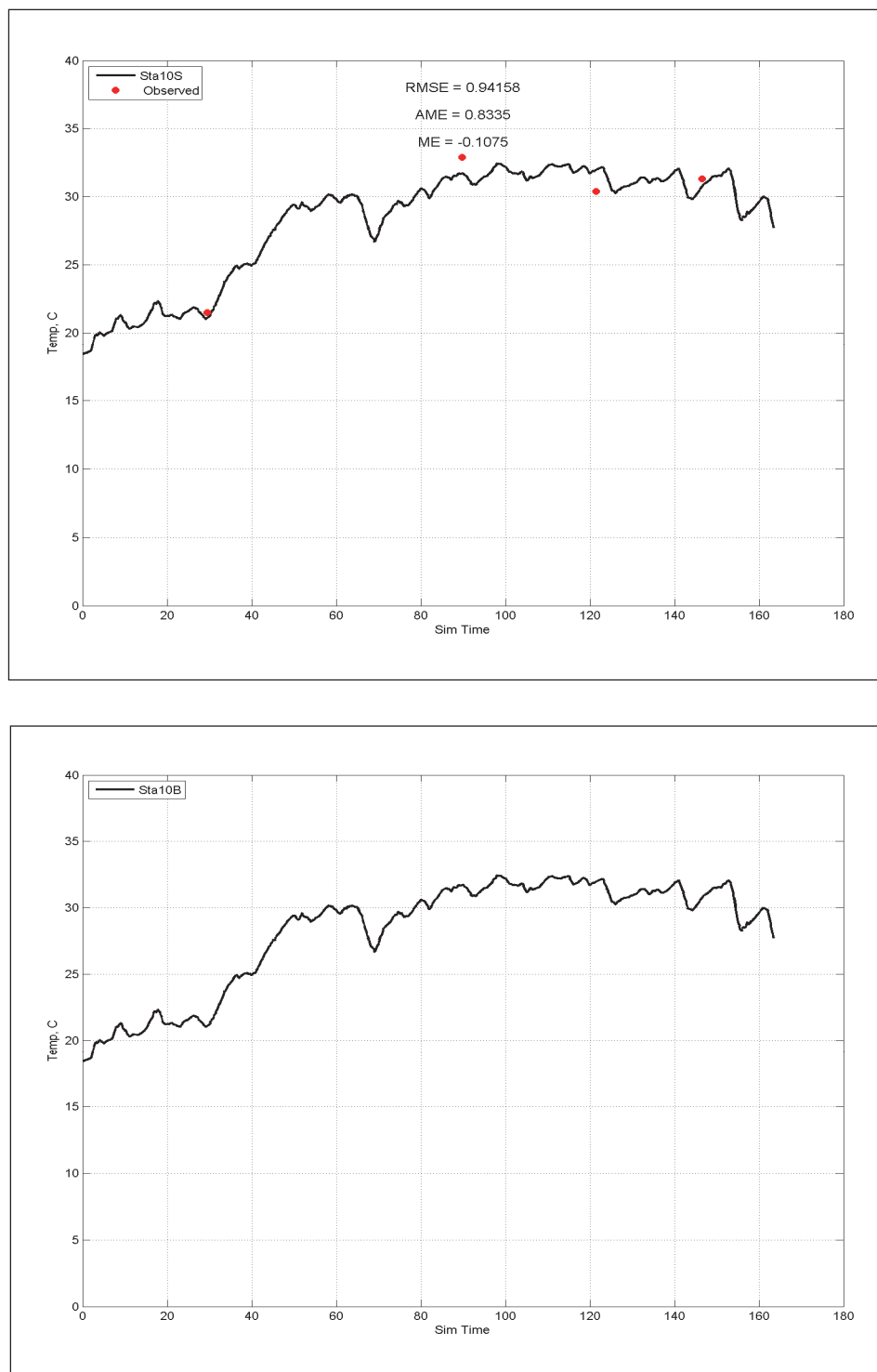
Figure E-55. Calibration results for temperature at Station 10 for surface layer (upper) and bottom layer (lower).
