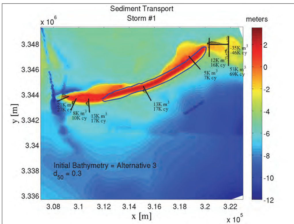
Figure J-2. Alternative 3 Restored conditions for Storm #1; d_{50} = 0.30 mm; With borrow pit.
