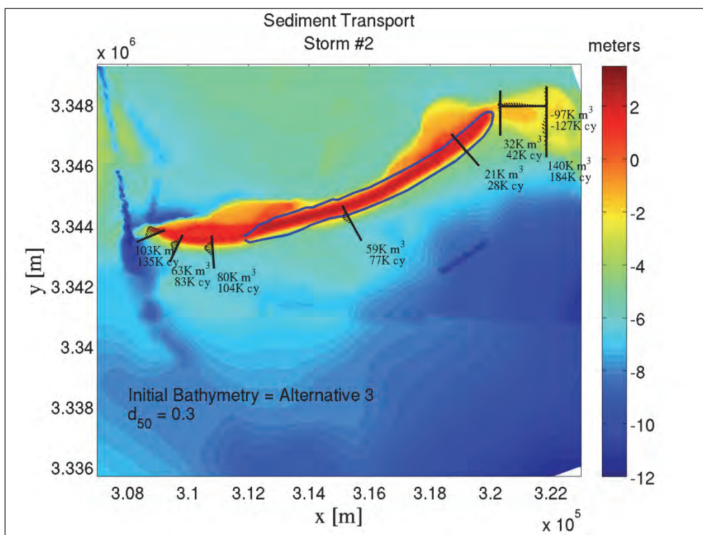
Figure J-4. Alternative 3 Restored conditions for Storm #2; d_{50} = 0.30 mm; With borrow pit.
