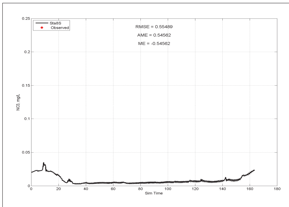
Figure E-47 Calibration results for \text{NO}_3 at Station 8 for surface layer (upper) and bottom layer (lower).
