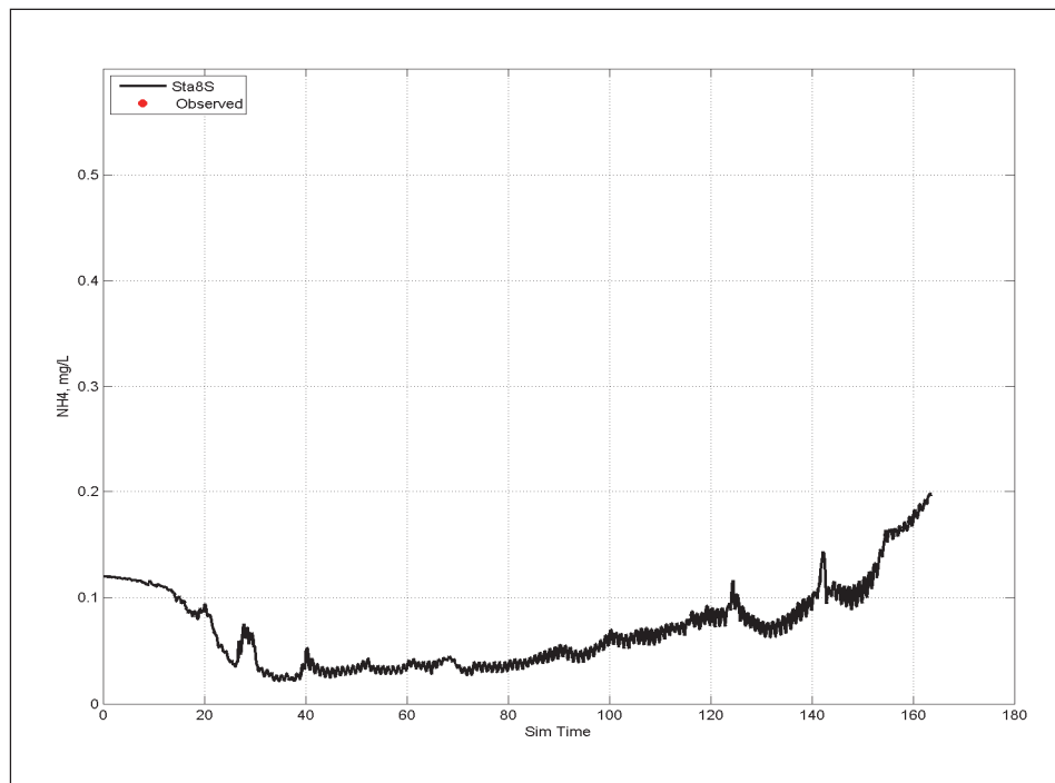
Figure E-46. Calibration results for \text{NH}_4 at Station 8 for surface layer (upper) and bottom layer (lower).
