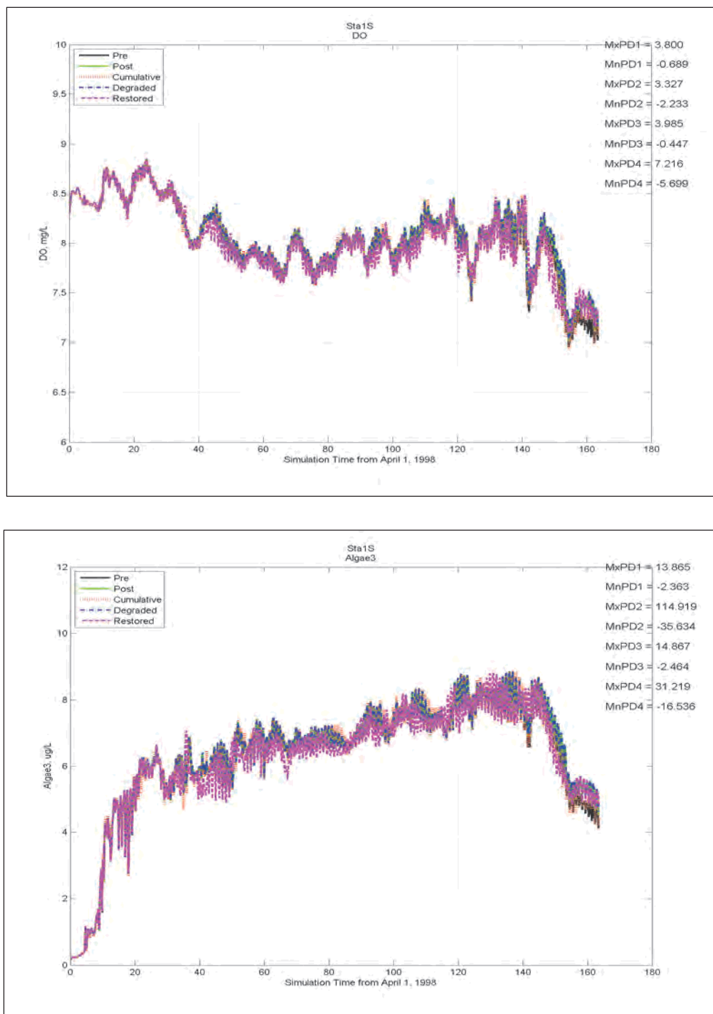
Figure E-61. Comparison of DO, Chlororphyll, and Salinity at Station 1 (Figure 5-2) for results from simulations representing Pre, Post, Restored, Degraded, and Cumulative conditions (continued).
