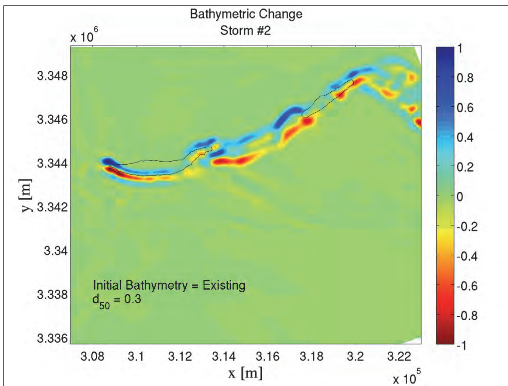
Figure J-9. Existing conditions for Storm #2; d_{50} = 0.30 mm.
