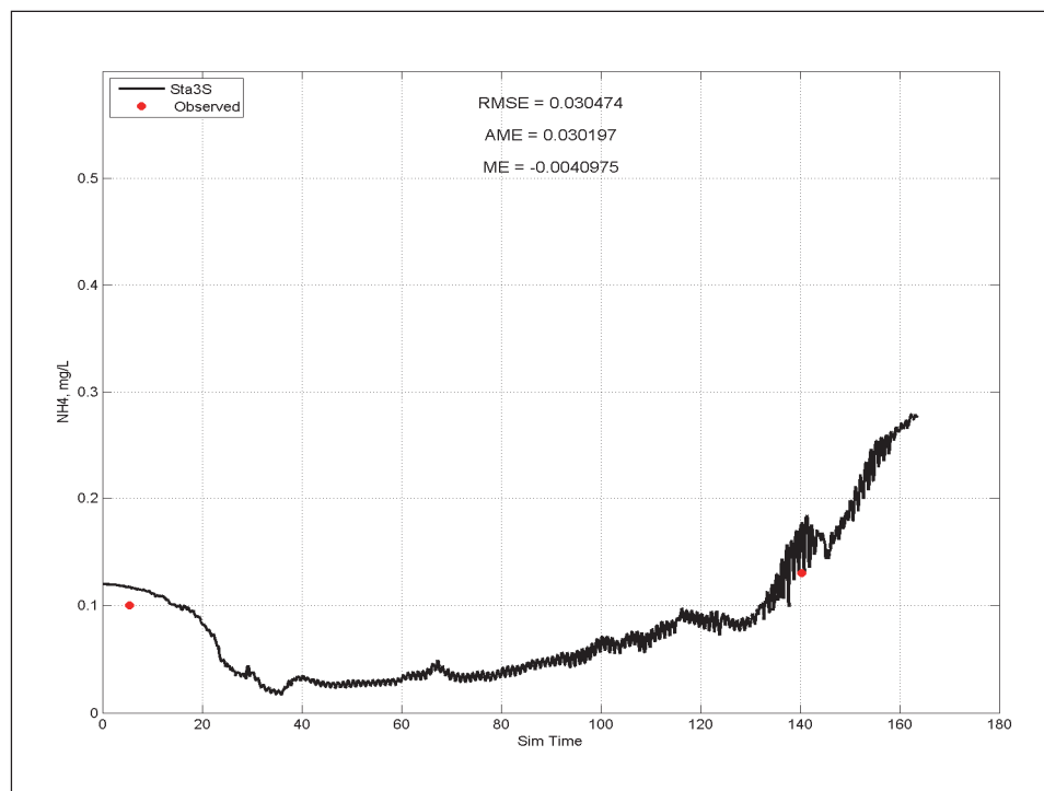
Figure E-16. Calibration results for \text{NH}_4 at Station 3 for surface layer (upper) and bottom layer (lower).
