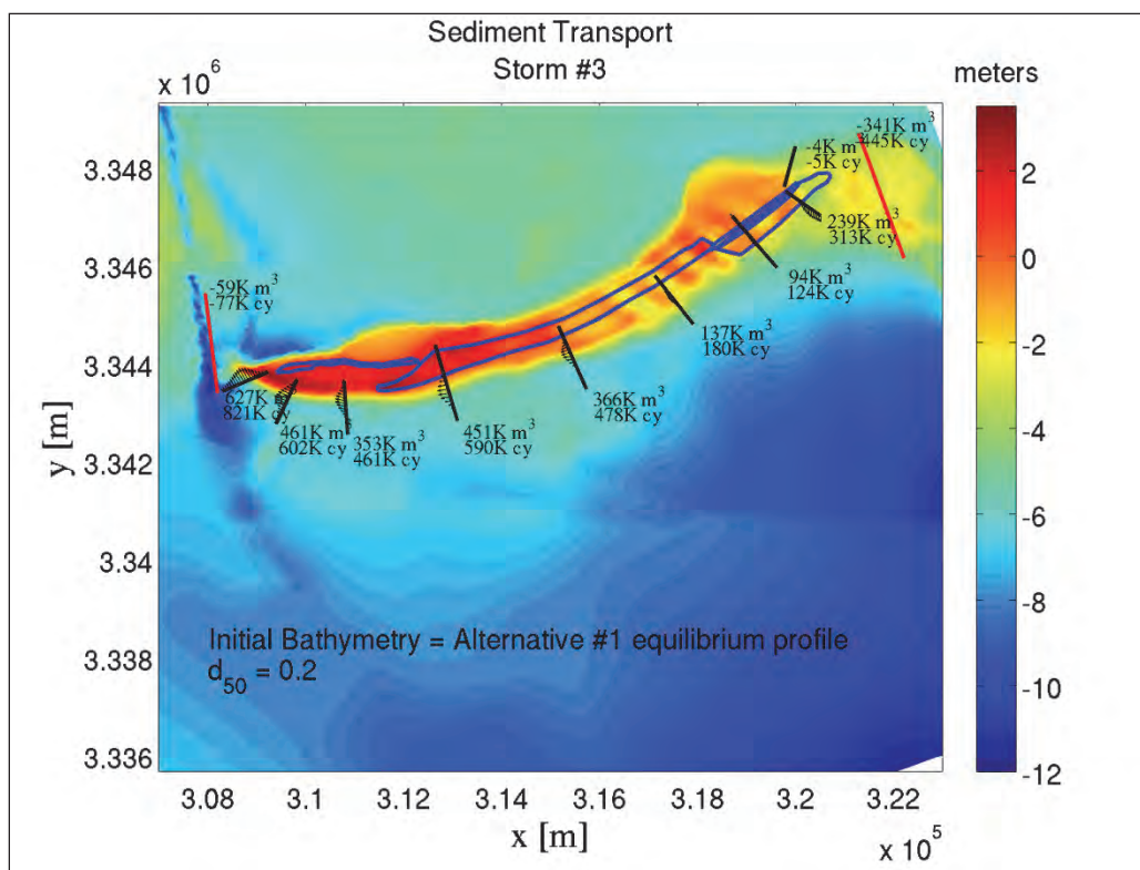
Figure G-19. Alternative #1 Restored conditions for Storm #3; Template A; Without borrow pits.
