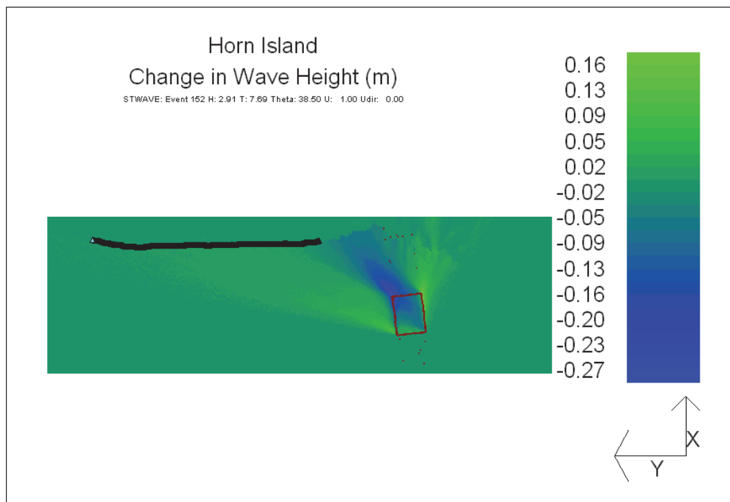
Figure 8-27. Wave height change (dredged – existing) for incident wave of H = 2.91 m, T = 7.69 sec and \Theta = 38.50 deg.
