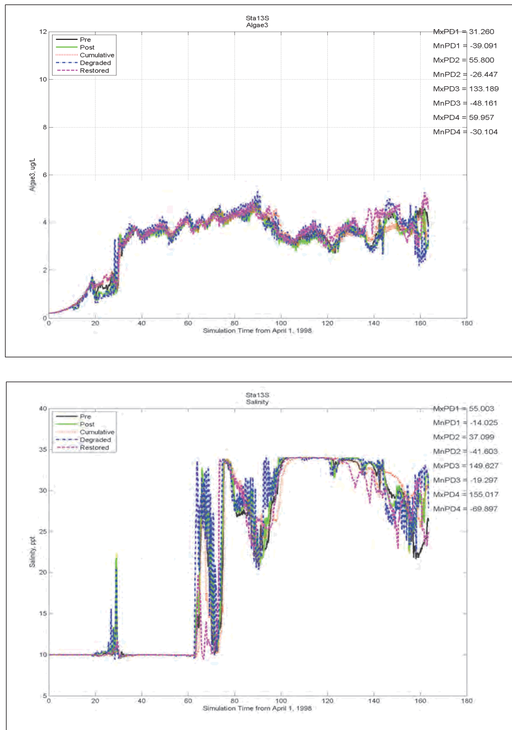
Figure E-70 Concluded.
