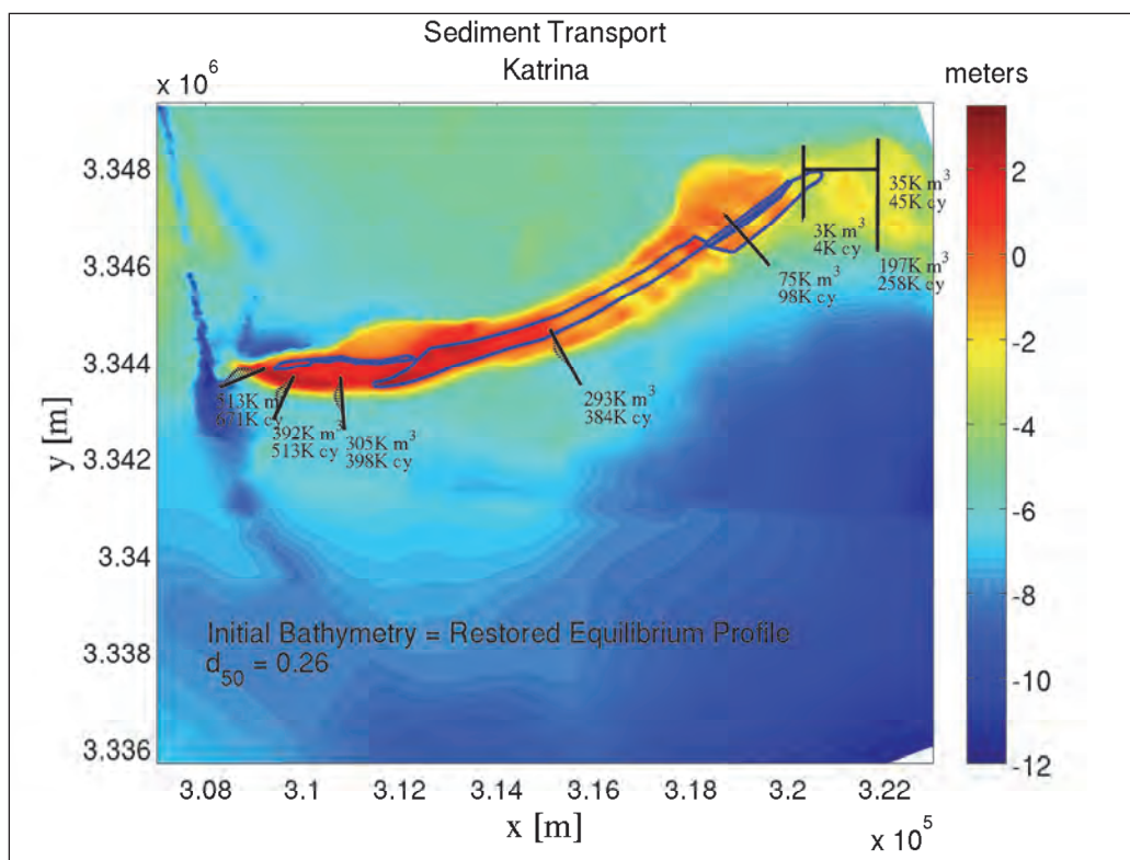
Figure I-6. Restored conditions for Katrina; d_{50} = 0.26 mm (Template #2); Without borrow pits.
