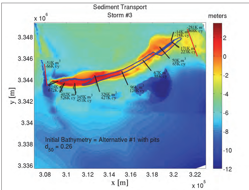
Figure G-17. Alternative #1 Restored conditions for Storm #3; Template B; With borrow pits.
