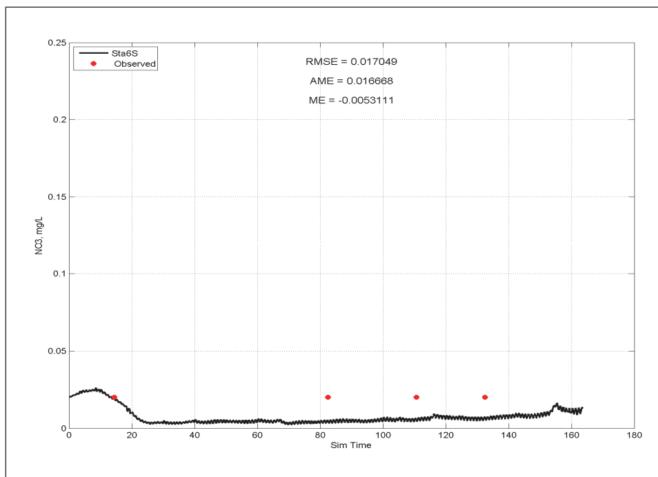
Figure E-35. Calibration results for \text{NO}_3 at Station 6 for surface layer (upper) and bottom layer (lower).
