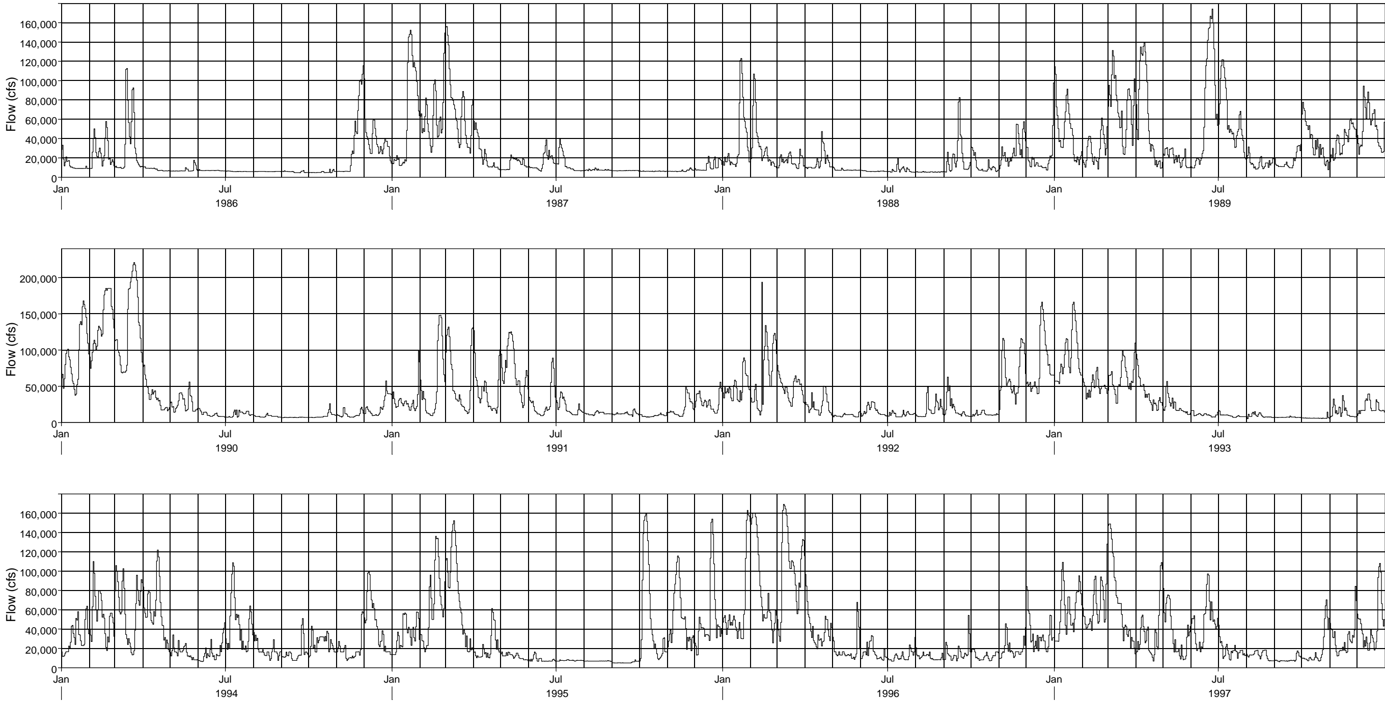
ALABAMA-COOSA-TALLAPOOSA RIVER BASIN WATER CONTROL MANUAL MILLERS FERRY LOCK AND DAM AND WILLIAM "BILL" DANNELLY LAKE AVERAGE DAILY DISCHARGE HYDROGRAPHS
