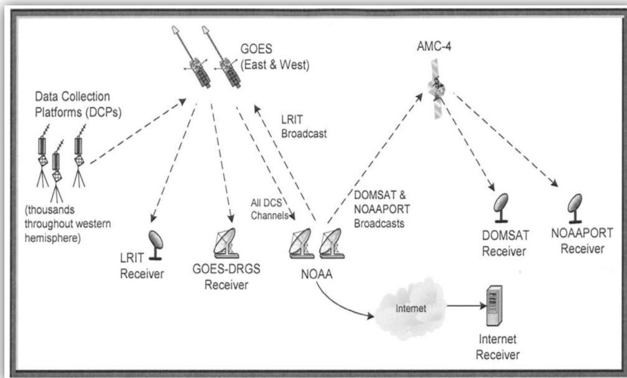
Figure 5-3. Typical Configuration of the GOES System
