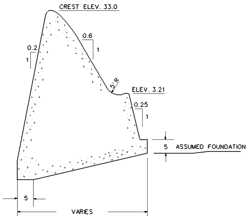
TYPICAL SECTION FIXED CREST SPILLWAY
