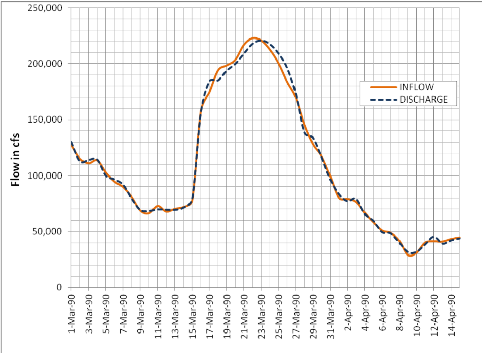
ALABAMA-COOSA-TALLAPOOSA RIVER BASIN WATER CONTROL MANUAL MILLERS FERRY LOCK AND DAM AND WILLIAM "BILL" DANNELLY LAKE INFLOW OUTFLOW POOL HYDROGRAPHS FLOOD OF MARCH 1990
