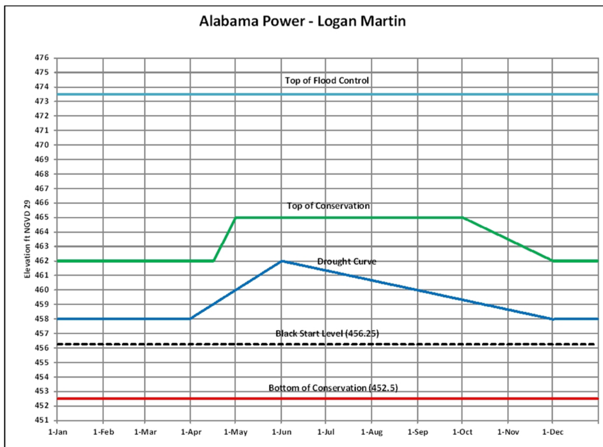
Figure 8. Logan Martin Lake Guide Curve
