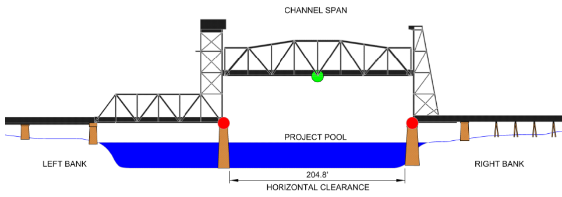
LOOKING DOWNSTREAM VIEW (OPEN)
