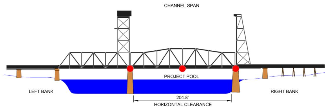
LOOKING DOWNSTREAM VIEW (CLOSED)
