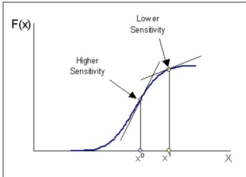
Figure A-5a. Hypothetical 2-D response surface for Y given one input variable: Y=F(X) . The sensitivity of Y with respect to X is calculated as the slope at a specific point on the surface (x^0, x^1) , or the partial derivative, \partial Y/\partial X_i .
