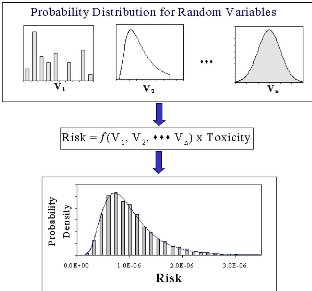
Figure 1-2. Conceptual model of Monte Carlo analysis. Random variables ( V_1, V_2, \dots, V_n ) refer to exposure variables (e.g., body weight, exposure frequency, ingestion rate) that are characterized by probability distributions. A unique risk estimate is calculated for each set of random values. Repeatedly sampling ( V_i ) results in a frequency distribution of risk, which can be described by a PDF. In human health risk assessments, the toxicity term should be expressed as a point estimate. In ecological risk assessment (see Sections 1.4 and 1.4.1) the toxicity term may be expressed as a point estimate or as a probability distribution.
