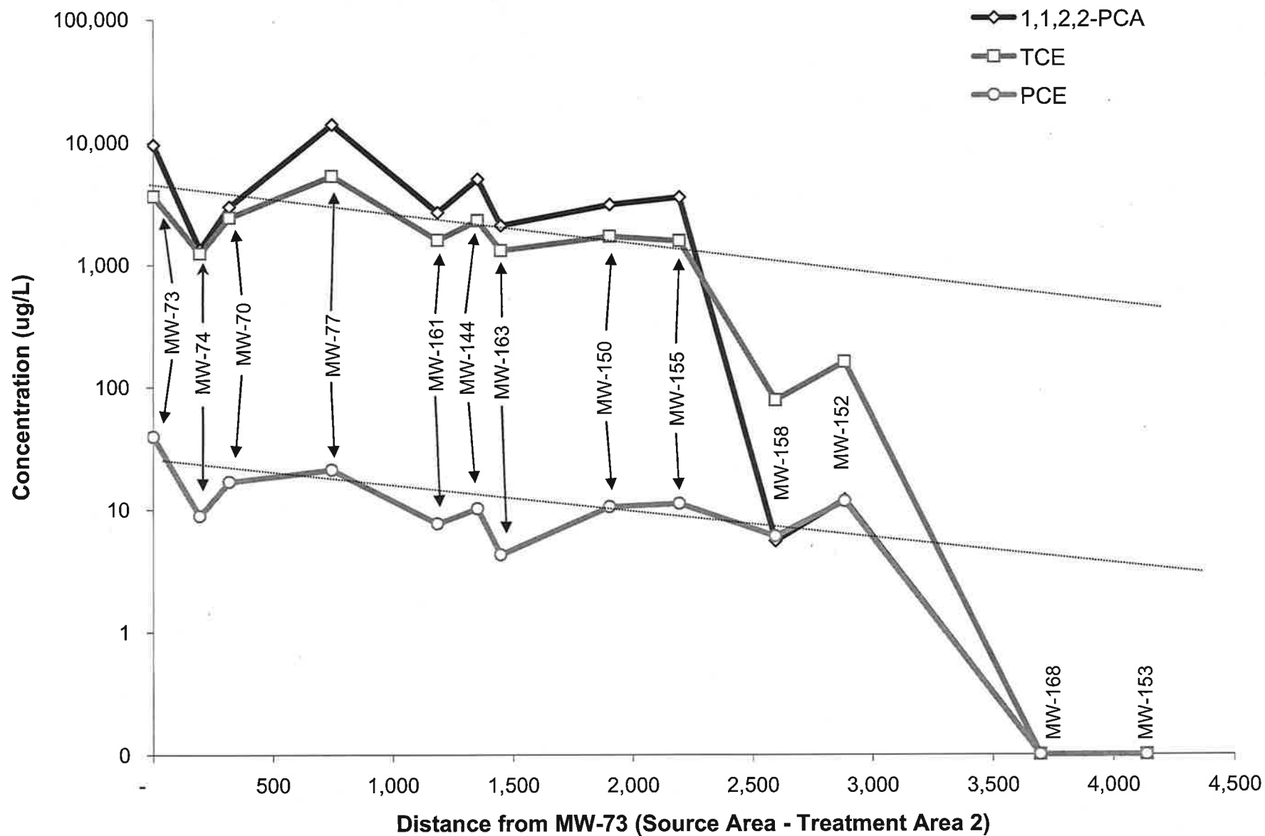
Figure 2-3 CVOC Concentrations Along Off-Depot Plume Centerline Memphis Depot Dunn Field
