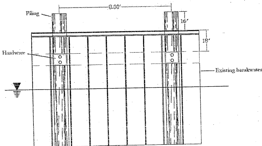
Wall Detail
