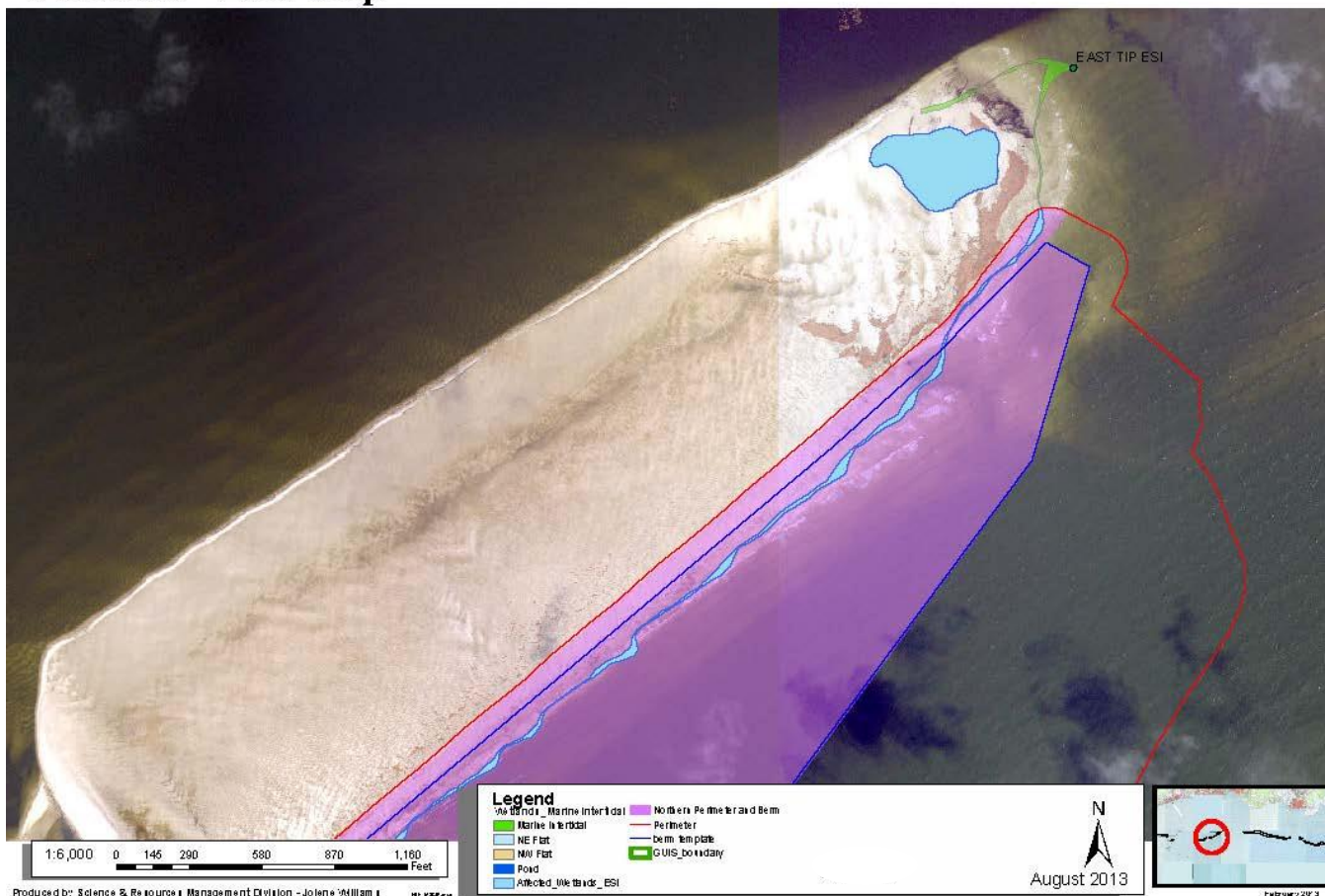
Figure 1-9. Sand placement east end of East Ship Island.
