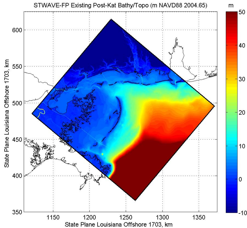
Figure 2-1. STWAVE-FP Existing Post-Katrina wave domain for March-June 2010 simulations.
