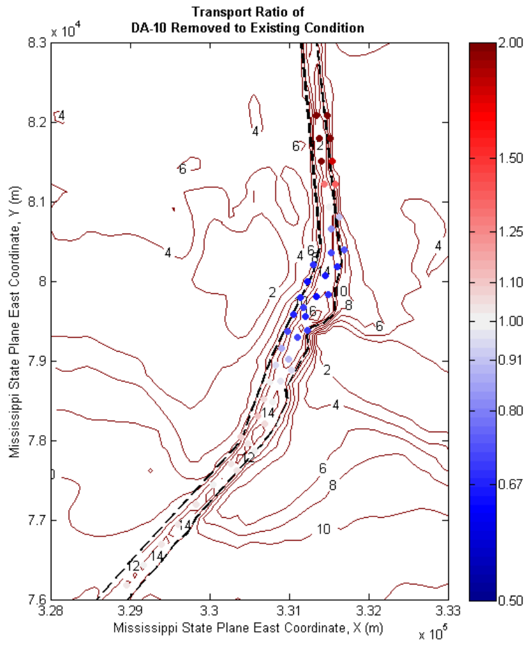
Figure 4-7. Ratio (removed/existing) of sediment transport magnitude within the navigation channel. Contours indicate bathymetry in meters relative to Mean Sea Level.
