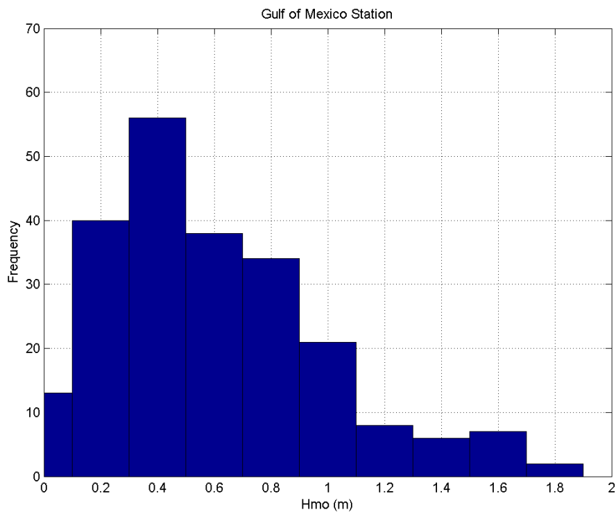
Figure 2-19. Histogram of the Measured H_{m0} (m) at the Gulf of Mexico Station.
