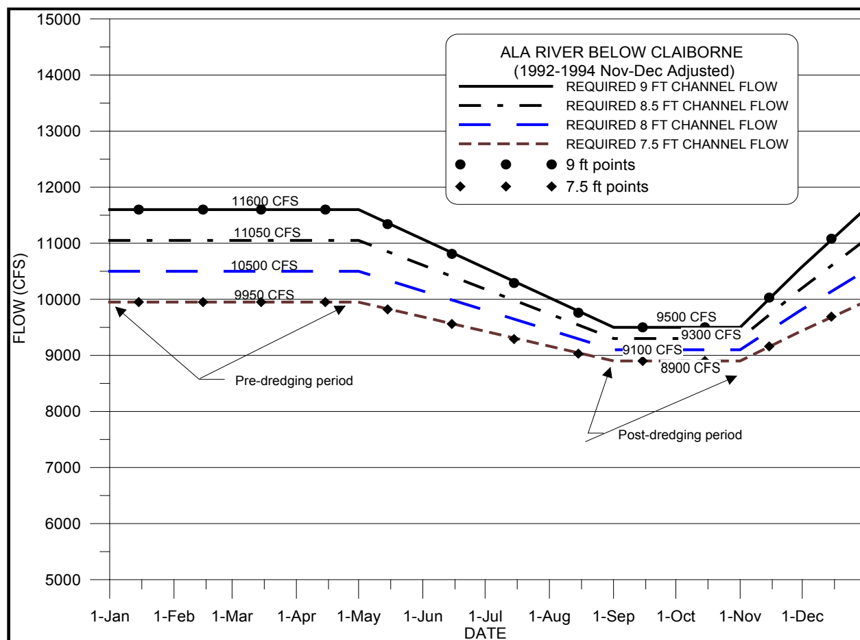
Figure 7-1. Flow-Depth Pattern (Navigation Template) Using 2004 – 2010 Survey Data
