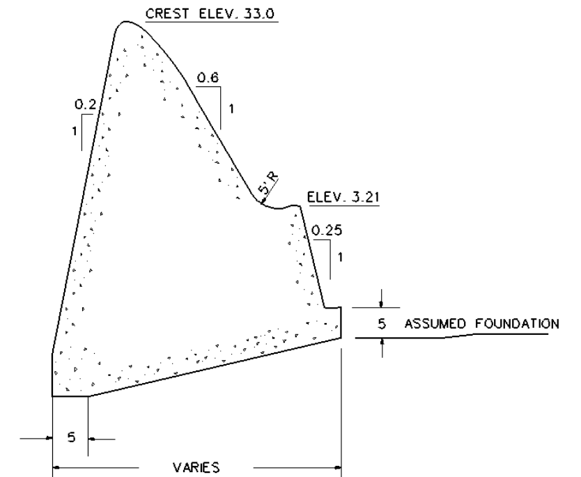
TYPICAL SECTION FIXED CREST SPILLWAY
