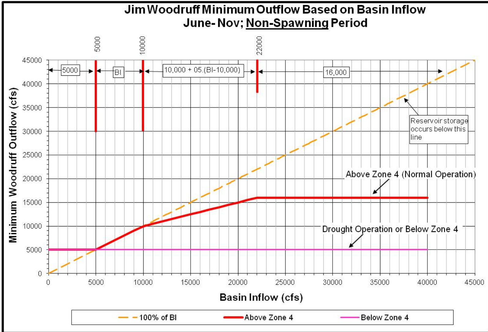
Figure 7-3. Minimum Woodruff Discharge during Non-Spawning Season
