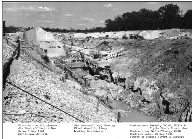
Figure 3-2. Construction of the Monolith, Circa May 1951
