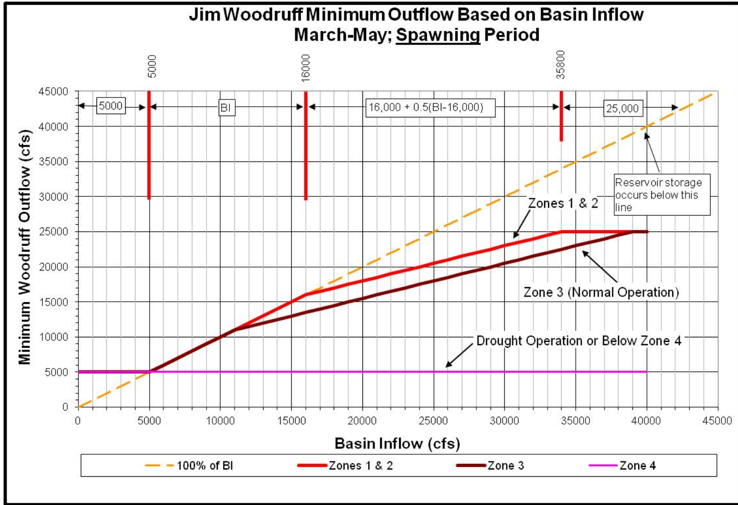
Figure 7-2. Minimum Woodruff Discharge during Spawning Season
