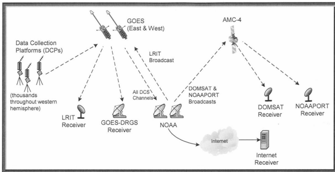
19 20 Figure 5-3. Typical Configuration of the GOES System
