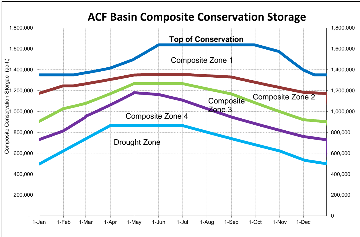
Figure 7-1. ACF Basin Composite Conservation Storage
