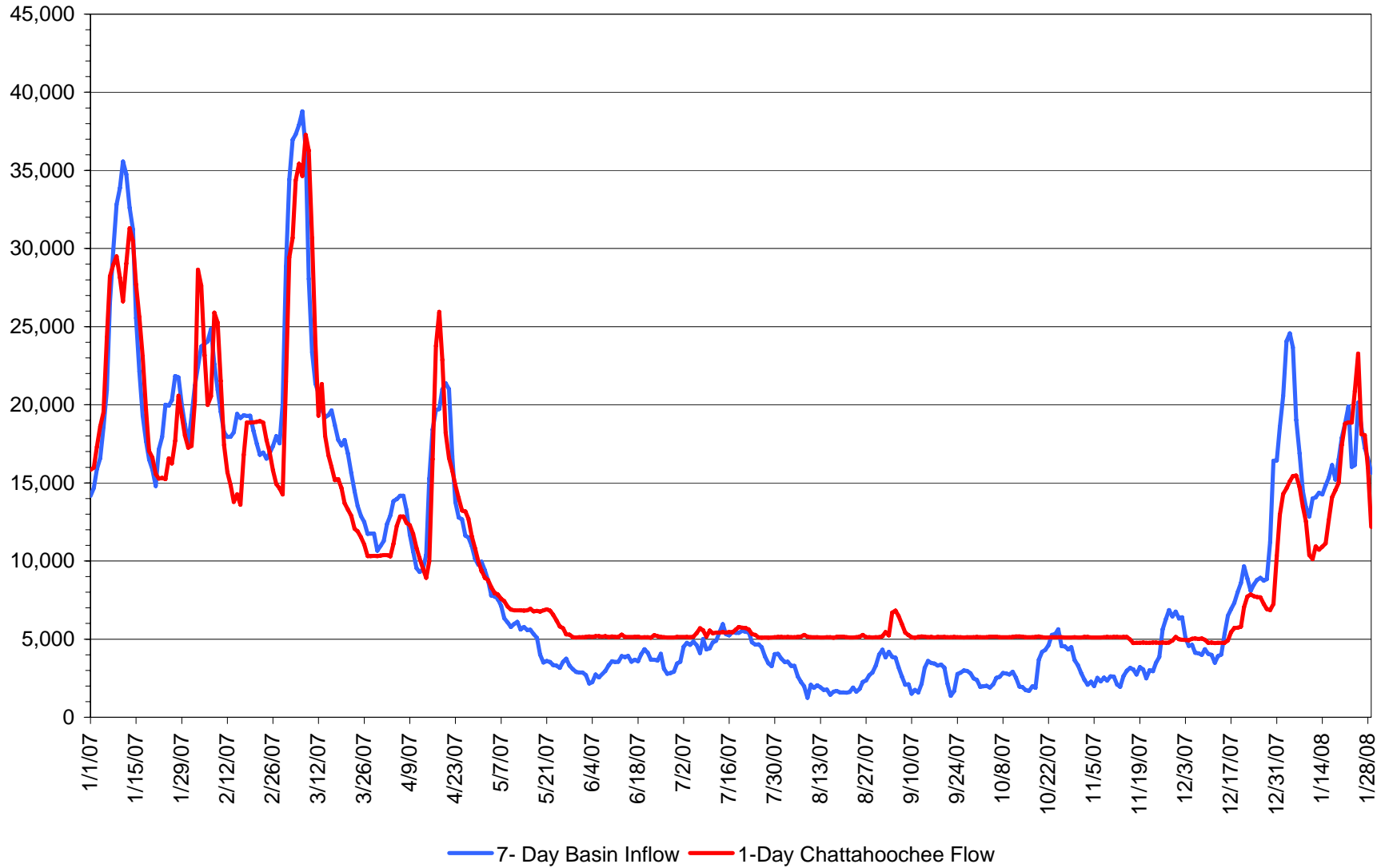
7 day Moving Average Basin Inflow v. 1 day Discharge at Chattahoochee Gage
